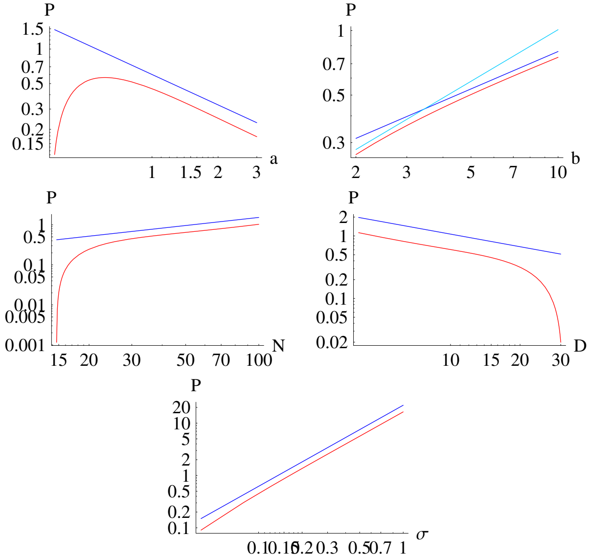
Figure 1: The equation of state of the PBBs in terms of system parameters. The plots indicate universal power laws as p \sim a^{-0.88} b^{0.8} \sigma^{1.55} \left(\frac{N}{D}\right)^{0.67} . In terms of the second Virial coefficient, the power law changes to p \sim b^{0.58} for larger bs .
