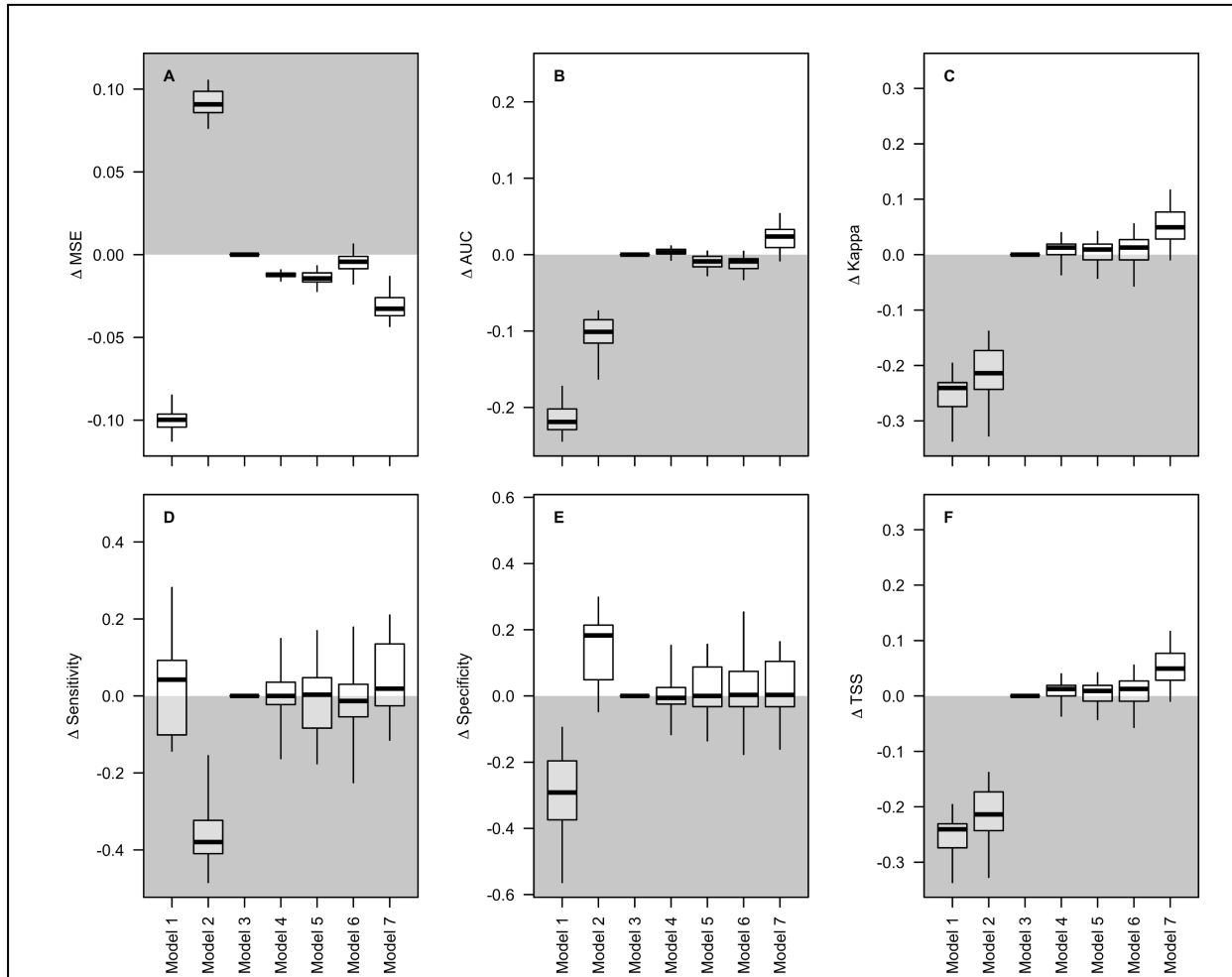
Figure 3. Differences in predictive performance metrics for the encounter rate models 1-7 against balanced and subsampled eBird data from 2017. Metrics are compared to the performance from model 3 and the y-axis values show differences relative to model 3. The white halves of the plots indicate where model performance is better than model 3. The grey halves of the plots indicate where model performance is worse than model 3. Model 3 uses all the data in a random forest encounter rate model. Model 7 is the random forest encounter rate model using complete checklists, spatial subsampling, effort variable filters, and effort variables as covariates. The validation metrics are calculated for 25 different model runs. For details of models 1-7 see Table 1 and the text. Boxes show the median, the interquartile range, and whisker ends denote the extremes of the distributions.
