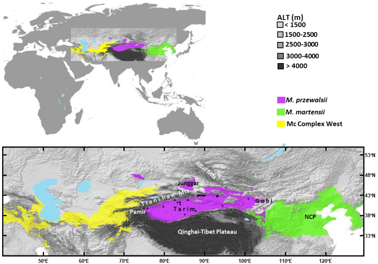
Figure 3. Ecological niche models of Mesobuthus scorpions. Potential distribution areas for the Przewalski's scorpion ( M. przewalsii , purple) is shown together the Chinese scorpion ( M. martensii , light green) and other species of the M. caucasicus complex (Mc Complex West, yellow). The entire Tarim Basin and adjacent Gobi region are suitable for survival of M. przewalsii . No area to the west of the Tianshan Mts and the Pamir Plateau is suitable for M. przewalsii , and similarly no area to the east of the Tianshan Mts and Pamir Plateau is suitable for other species of the M. caucasicus complex. There are overlaps in predicted suitable distribution areas between M. przewalsii and M. martensii along the northeast edge of the Qinghai-Tibet Plateau. The suitable areas in the Junggar Basin and two the north of the Tianshan Mts are due to over prediction of the model, because M. przewalsii does not occur in these regions. Ecological niche model for M. martensii was adopted from Shi et al. 2007.
