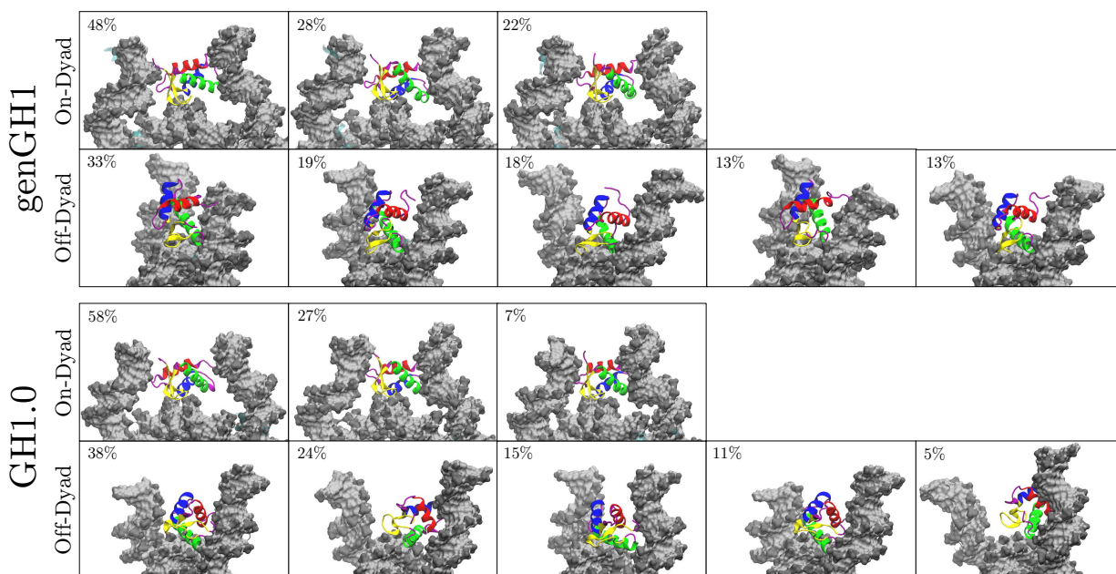
Figure 4: Representative snapshots of clusters for linker histones genGH1 and GH1.0 in both the on- and off-dyad binding modes. Shown are clusters totalling at least the top 90% of frames analyzed. The respective percentage of each cluster is provided in the top left-hand corner of each snapshot.
