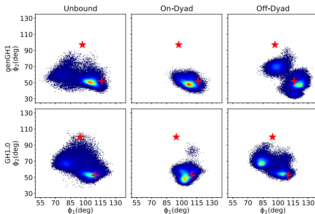
Figure 2: Flexibility of the \beta -loop using \phi -angles inspired by a previous study. 53 Shown are 2D-histograms of \phi_2 versus \phi_1 angles (deg) in the unbound (left), on-dyad (middle), and off-dyad (right) states. Density ranges from blue (lower) to red (higher). The red cross corresponds to the initial values of the closed-state linker histone, while the red star corresponds to the open-state values.
