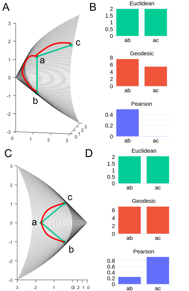
Fig. 2: Motivating functional connectivity geometry. (A) Identical Euclidean distance does not imply identical geodesic distance. (C) Identical geodesic distance can yield very different Pearson dissimilarity. (B, D) Comparison of distances/dissimilarity ab and ac in (A) and (C), respectively. Distances/dissimilarity cannot be compared across measures because their units are arbitrary.
