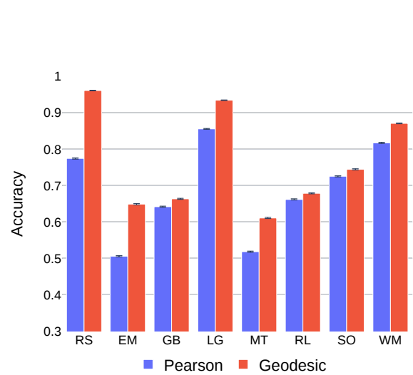
Fig. 3: Participant identification for the eight conditions using the geodesic distance and Pearson dissimilarity. Training and testing data were from the same condition. Accuracy improved using the geodesic distance on each condition. Error bars indicate standard error of the mean across bootstrap iterations. Abbreviations: EM, emotion processing; GB, gambling; LG, language; MT, motor; RL, relational processing; RS, resting-state; SO, social cognition; WM, working memory.
