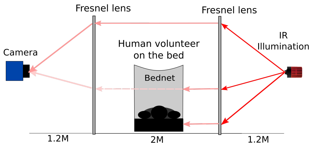
(a) Backlit recording setup
