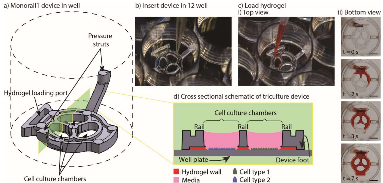
Figure 1. Overview of Monorail1 device design features and operation. a) Monorail1 device (dashed lines represent the well of a 12-well cell culture plate). b) The device is loaded into the well of a standard 12-well cell culture plate using forceps. c) Hydrogel is loaded into the hydrogel loading port with a standard pipet, as seen from i) above the well plate or ii) below the well plate. Hydrogel is tinted with red dye for visualization purposes. ii) Bottom view images of the gel-precursor solution patterning progression at four timepoints (video is included in the SI). Scale bars: 5 mm d) Schematic of the device in cross-section depicting distinct cell types (blue, green) in different culture chambers that are separated by a hydrogel wall formed between the bottom of the rail and the base of the well.
