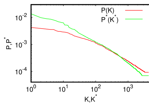
Fig. S.1. PageRank P(K) and CheiRank P^*(K^*) for the single protein network.
