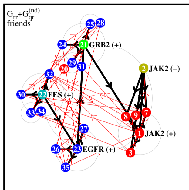
Fig. 4. Network of friends for the subgroup of nodes given in Table 1 corresponding to injection at EGFR P00533 (+) and absorption at JAK2 O60674 (-) constructed from the matrix G_{rr} + G_{qrd} using 4 top (friends) links per column (see text for explanations).
