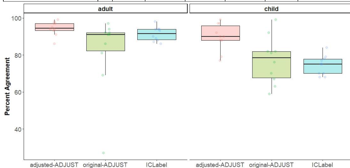
Figure 2. Box plots showing the distribution of the percent agreement scores for children and adults further split up by each algorithm (adjusted-ADJUST, original-ADJUST, or ICLabel). Each dot represents a score.
