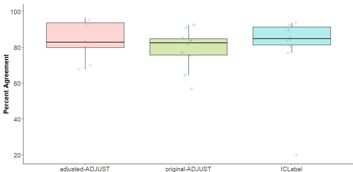
Figure 3. Box plots showing the distribution of the percent agreement scores for infants further split up by each algorithm (adjusted-ADJUST, original-ADJUST, or ICLabel). Each dot represents a score.
