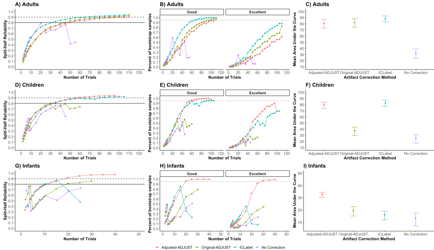
Figure 6. Internal consistency reliability of the mean P1 ERP amplitude in adults and alpha power in infants. Plots A, D, and G show the mean reliability across the 10,000 samples at each number of trials, n . Plots B, E, and H show the percentage of the resampling distribution that achieves good (left) and excellent (right) reliability. Plots C, F, and I show the average area under the curve of the reliability curves (plots B, E, and H) with the 95% CIs of the resampling distribution.
