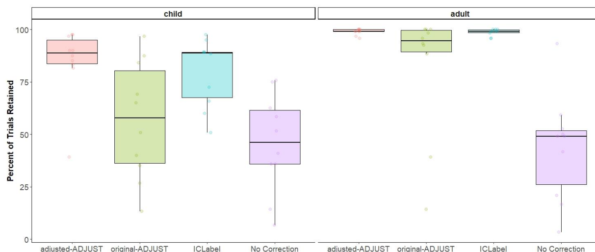
Figure 4. Box plots showing the number of trials retained after artifact rejection for each condition (adjusted-ADJUST, original-ADJUST, ICLabel, or No Correction) further split up by age group (child or adult). Each dot represents a score.
