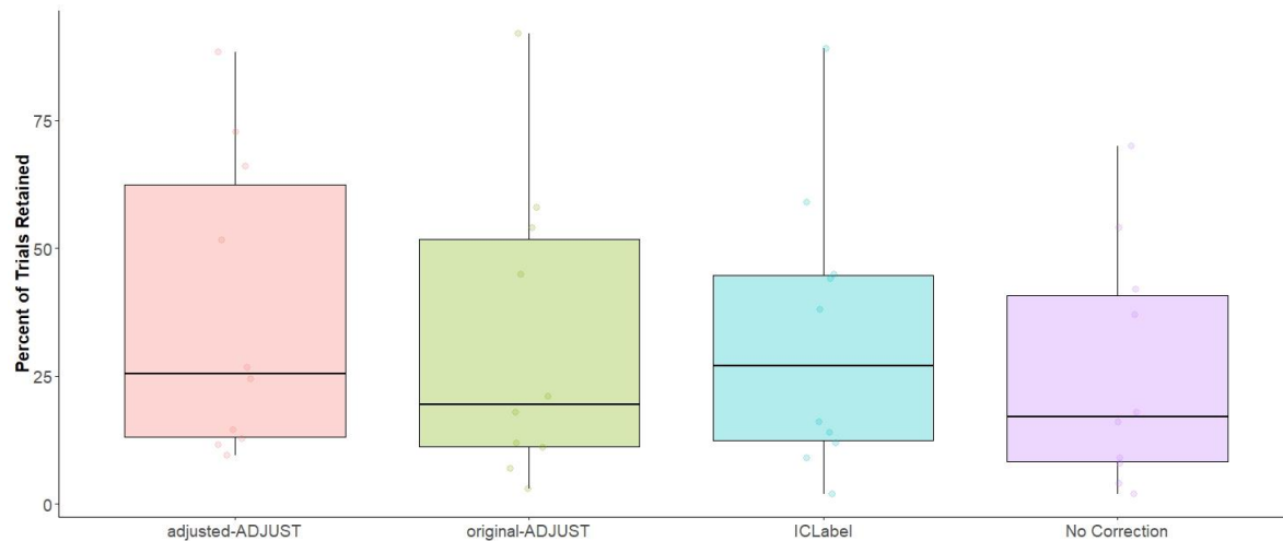
Figure 5. Box plots showing the percent of trials retained after artifact rejection for each condition (adjusted-ADJUST, original-ADJUST, ICLabel, or No Correction) for infants. Each dot represents a score.
