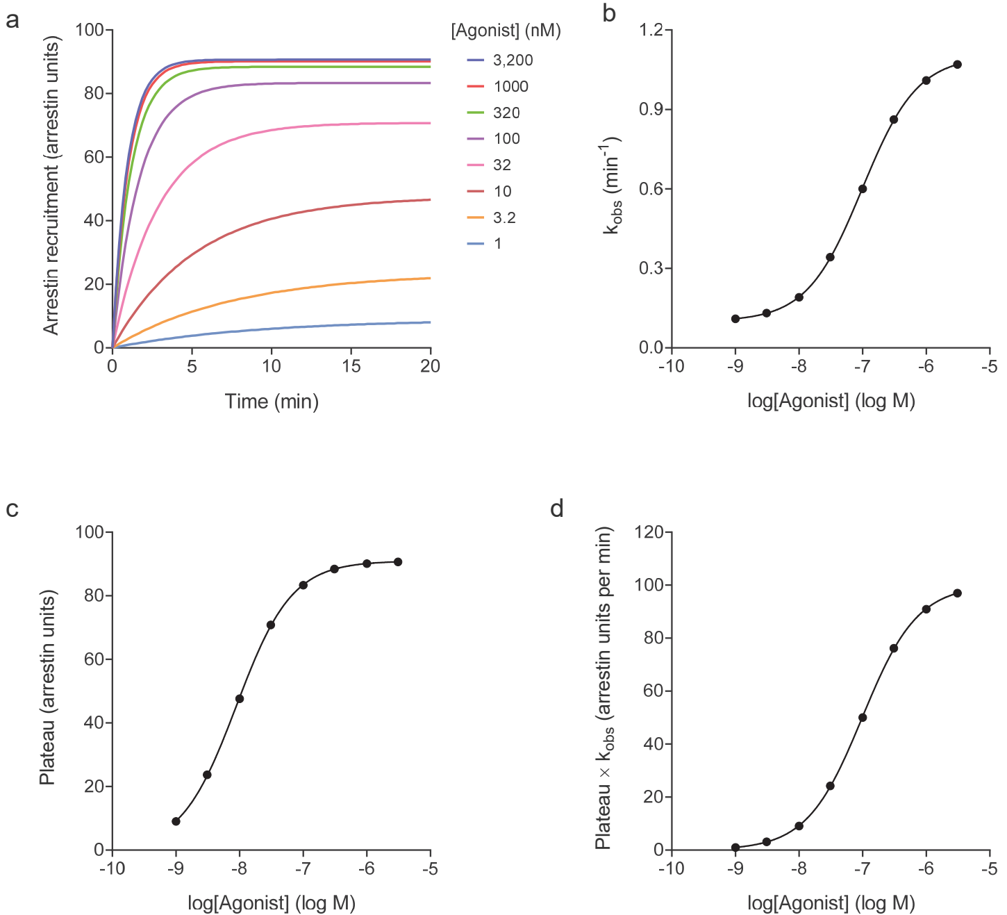
Supplementary Figure S3. Simulated arrestin recruitment data. The arrestin recruitment model (Appendix) was used to simulate the time course of arrestin recruitment to a GPCR stimulated by agonist ligand. Time course data (a) were simulated using equation (1), assuming receptor is in excess over arrestin, for a range of concentrations of agonist. From these data the observed rate constant k_{obs} and Plateau can be calculated using equation (3). The calculated values are plotted versus the agonist concentration (b, k_{obs} ; c, Plateau). Note the value of both parameters increases as the ligand concentration increases. The curves are fits to a sigmoid dose-response equation. Finally, the initial rate of recruitment at each concentration can be determined by multiplying the Plateau by k_{obs} . The resulting value is plotted against the agonist concentration (d). The data are then fit by the sigmoid dose-response equation to determine k_{\tau} ( k_{obs} \times \text{Plateau} at maximally-effective [A]) and agonist affinity for the receptor ( [A]_{50} ). Model parameter values used for the simulation were: K_A , 100 nM; [R]_{TOT} , 100 receptor units; [N]_{TOT} , 100 arrestin units; k_N , 0.01 receptor units ^{-1} min ^{-1} ; k_{-N} , 0.1 min ^{-1} . The calculated k_{\tau} value was 100 arrestin units.min ^{-1} .
