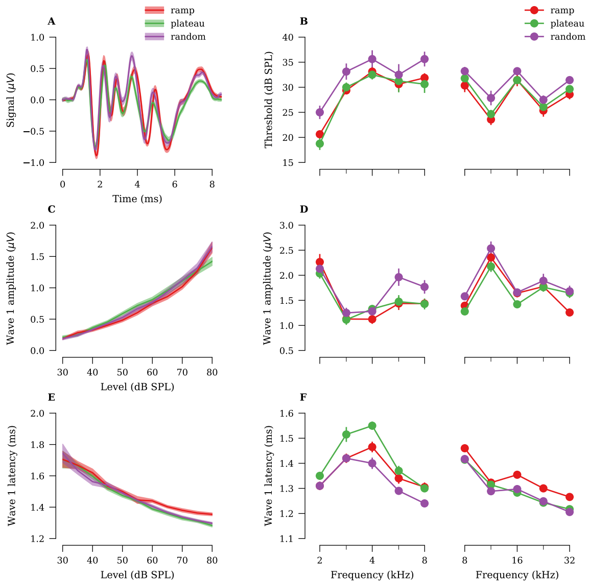
Fig. 5 Comparison of interleaved stimulus designs ( n = 8 ears from gerbil, n = 10 ears from mouse). A) Overlay of average ABR waveforms acquired using each design. Responses are to 16 kHz, 80 dB SPL, 80/s tone pips in mouse. B) Average ABR thresholds. C) Average ABR wave 1 amplitude vs. stimulus level for 16 kHz, 80/s tone pips. D) Average wave 1 amplitude at 80 dB SPL. E) Average ABR wave 1 latency vs. stimulus level for a 16 kHz, 80/s tone pip. F) Wave 1 latency at 80 dB SPL. Errorbars in all panels indicate \pm SEM
