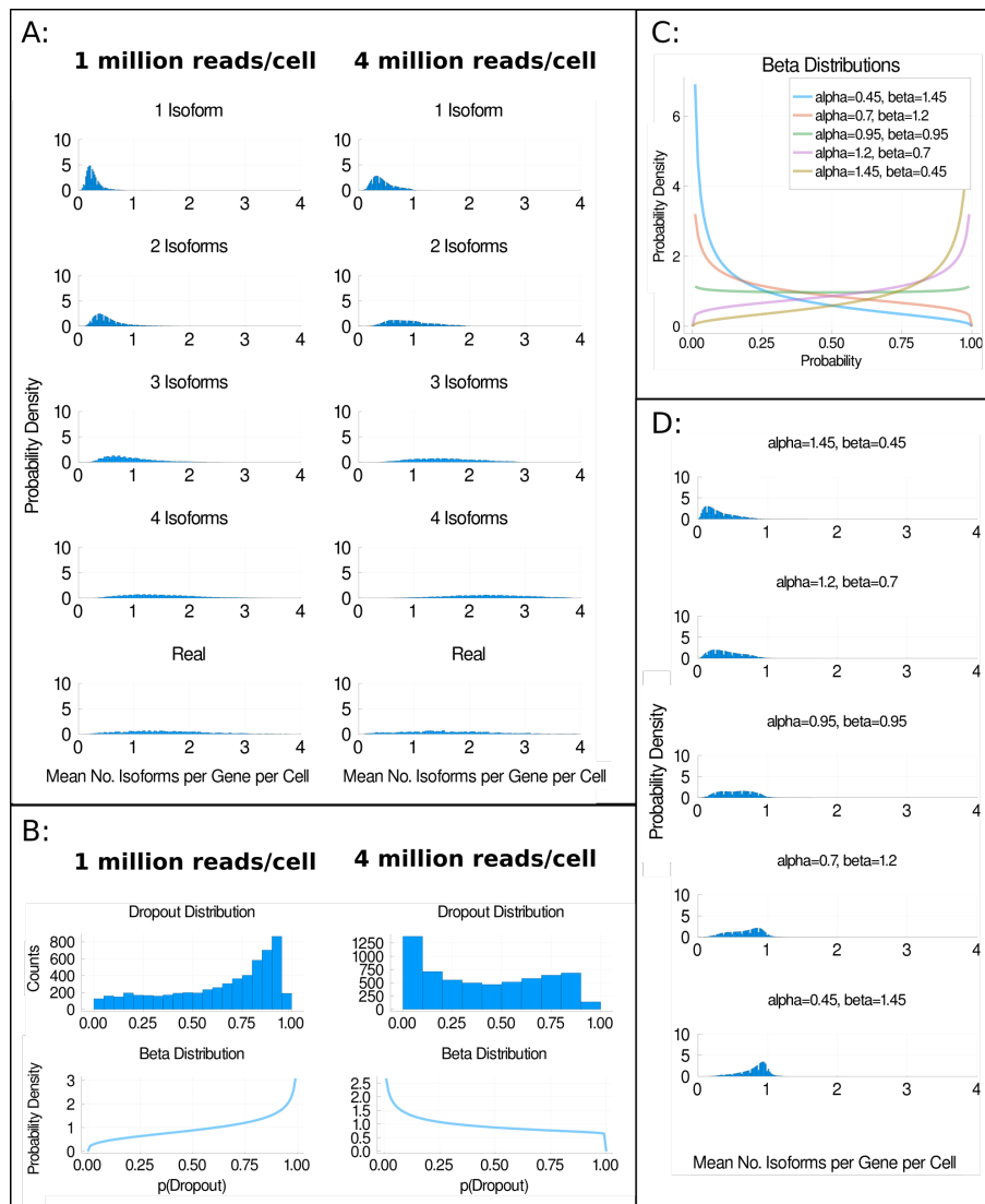
Figure 1: The impact of dropouts on isoform detection. a Distributions of the mean number of isoforms detected per gene per cell for H1 hESCs whose cDNA was split and sequenced at approximately 1 million reads per cell or 4 million reads per cell on average. b shows the distribution of the probabilities of dropouts ( p(\text{Dropout}) ) in each group and an approximation of these distributions using a Beta distribution. At 1 million reads per cell, \alpha = 1.31 and \beta = 0.74 in the approximated Beta distribution. At 4 million reads per cell, \alpha = 0.72 and \beta = 1.03 in the approximated Beta distribution. c shows five Beta Distributions from which dropout probabilities were sampled from in the simulations used to generate d . In d , the distribution of the mean number of isoforms detected per gene per cell is shown for simulations in which one isoform was produced per gene per cell. Each plot corresponds to a simulation in which dropout probabilities were sampled from one of the distributions shown in c . Plots shown in d are for H1 hESCs sequenced at 4 million reads per cell. See Supplementary Figure 1 for equivalent plots for the H9 hESCs.
