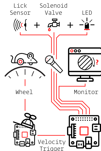
Figure 4.4: Hardware distribution for the distributed go/no-go task
