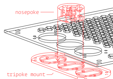
Figure 3.6: We have designed a basic set of easily-assembled hardware available on Autopilot's website .
