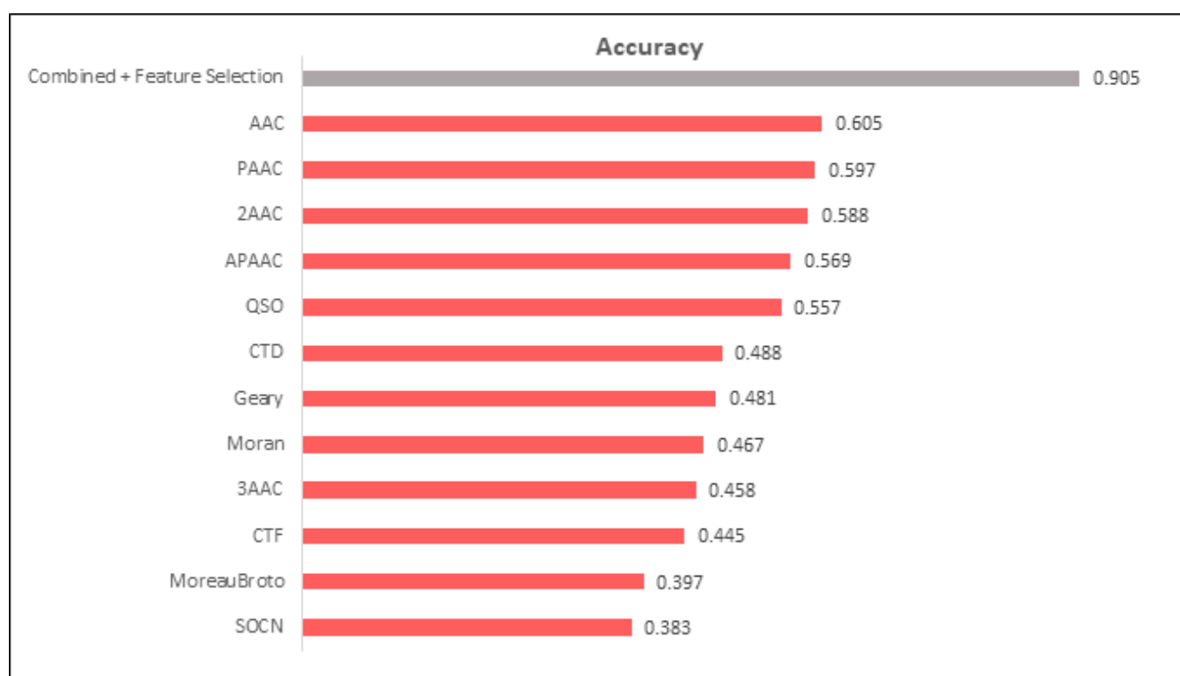
Figure 3 : Feature Importance Analysis. This chart represents the importance and relevance of each generated feature set with the task of thermal activity prediction. Mean of accuracy for the same model, trained with different feature sets, are provided and compared. This representation implies the importance of feature selection steps in order to obtain a better prediction performance.
