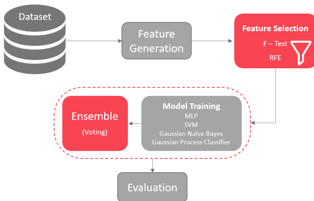
Figure 2 Schematic diagram of the workflow . The figure above illustrates the steps for the development and evaluation of proposed prediction model.
