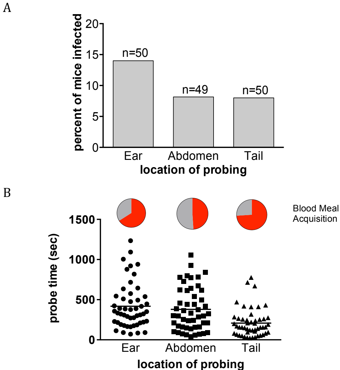
Figure 4. The anatomical location of mosquito probing does not impact the likelihood of malaria infection. Single-mosquito feeds were performed on the ear, abdomen or tail of mice and probe time and blood meal acquisition were recorded. Following this, salivary gland sporozoite loads were measured and mice were followed for blood stage malaria infection. (A) Percent of mice positive for malaria infection when probed-upon at the indicated location. n=total number of mouse-mosquito pairs in each group, pooled from 4 independent experiments with 10 to 15 mouse-mosquito pairs per group per experiment. The risk of infection is not statistically different between the three locations ( p=0.655 ). (B) Probe time and blood meal acquisition of mosquitoes placed on different anatomical locations. During the location feeds, mosquitoes were allowed to probe until they took a blood meal or became disinterested and flew away. Times to either of these endpoints were measured and were lower for mosquitoes placed on the tail compared to the abdomen and ear, by 45 to 50 percent respectively ( p<0.001 ). The percent of mosquitoes feeding on the ear, abdomen and tail that succeeded in obtaining a blood meal is shown in red in the pie charts and was 66%, 51%, and 74%, respectively. This difference did not reach statistical significance ( p=0.06 , Fisher's exact test).
