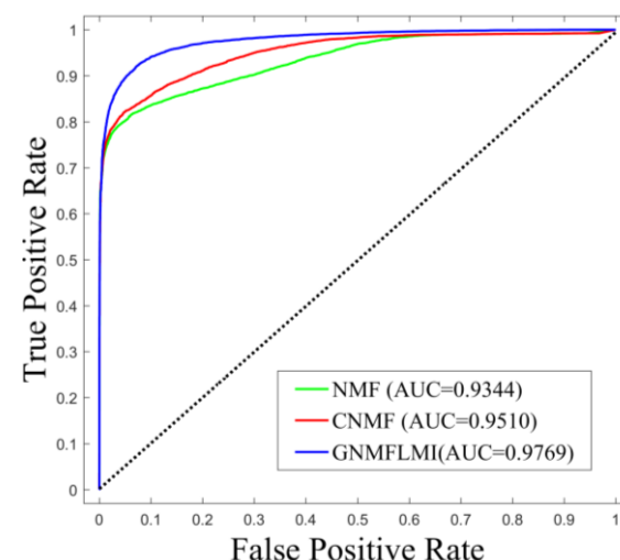
Fig. 5. The ROC curves of three methods.
