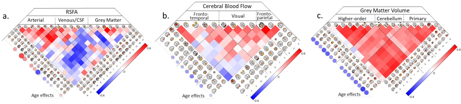
Figure 5 Independent component analysis spatial maps and correlation between subject loadings for RSFA (a), cerebral blood flow (b) and grey matter volume (c) datasets. The relationships between age and IC loadings are shown circles on the left hand-side of each correlation matrix, FDR-adjusted p -value of 0.05.
