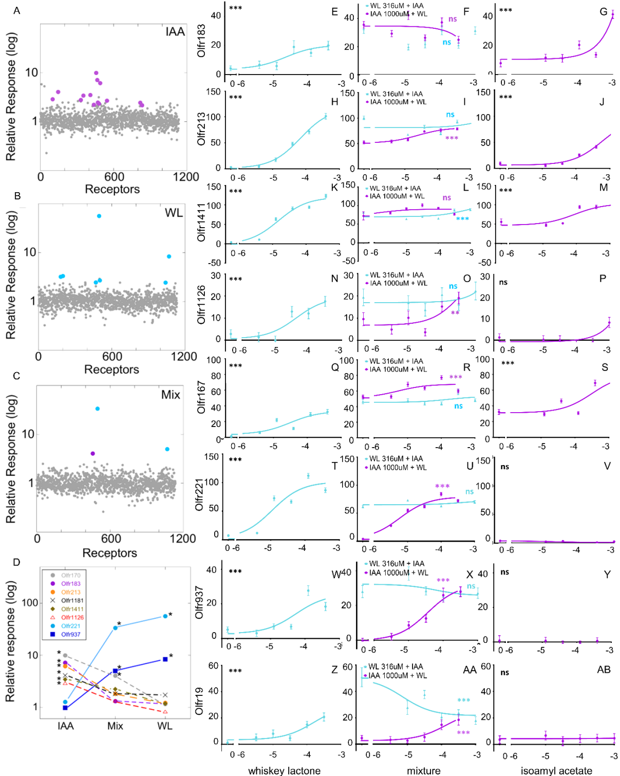
Figure 2. Odorant receptors responsive to isoamyl acetate (IAA) and whiskey lactone (WL). Of the more than 1,100 ORs and trace-amine associated receptors (TAARs) expressed in the mouse olfactory epithelium (shown in alphabetical order on the x-axis in A-C ), 14 ORs responded to 5% IAA (violet) in vivo ( A ) and 7 ORs responded to 50% WL (blue) in vivo ( B ). Only the 2 ORs highly responsive to WL and the 1
