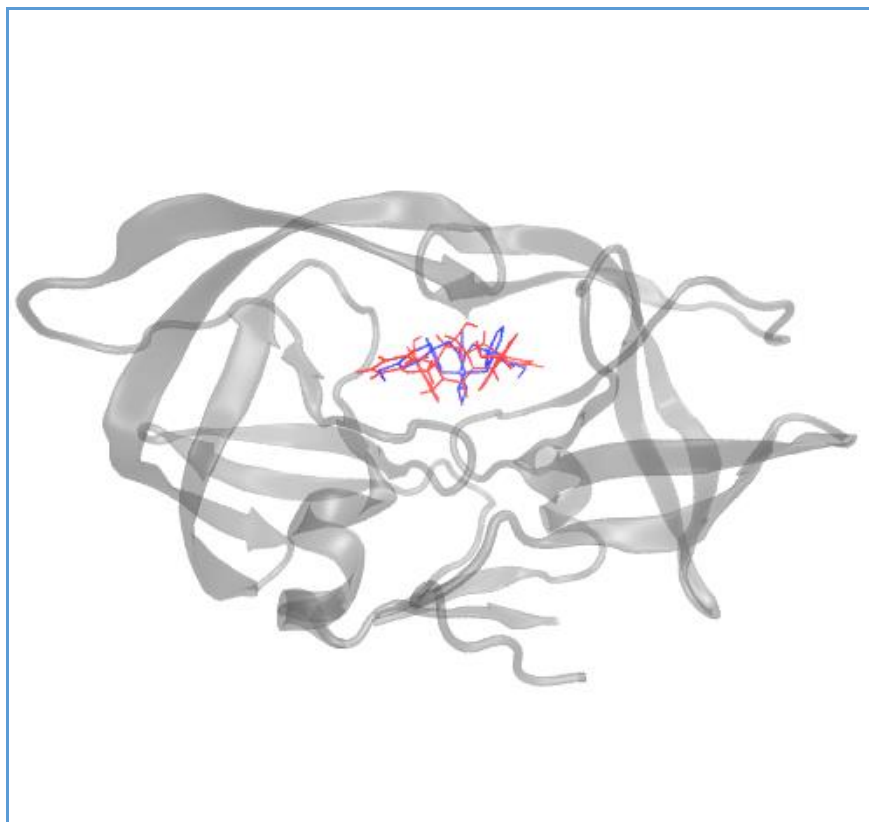
Figure S1. Docking ligand into HIV-1 protease. DMP (blue) is the co-crystalized ligand in HIV-1 protease (PDB code: 1QBS). Ligand A008 (red) is docked into the HIV-1 of 1QBS.
