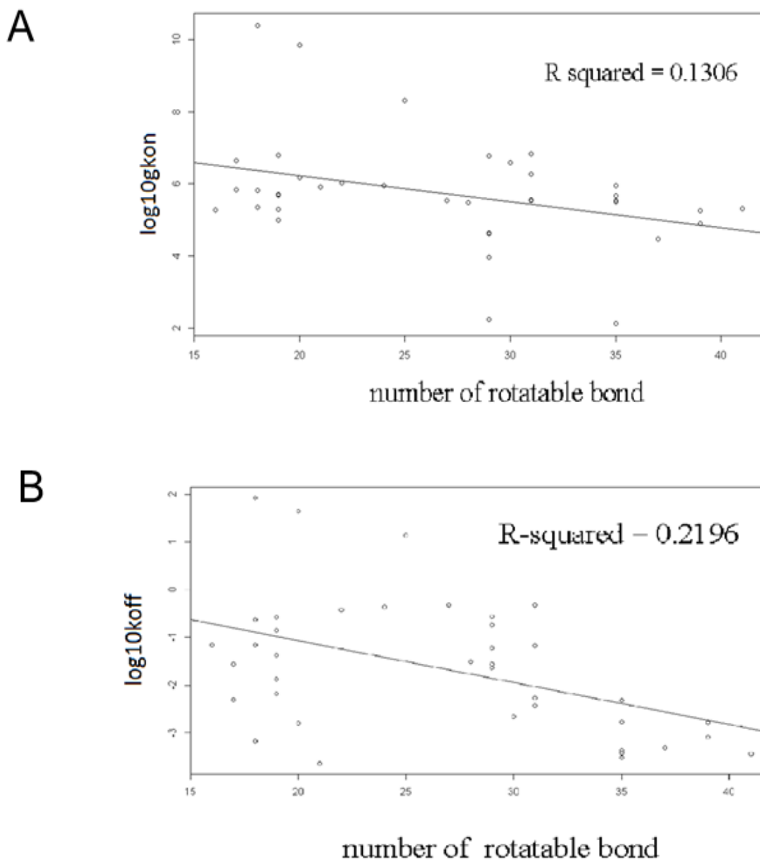
Figure S2. Number of ligand rotatable bond versus \log_{10}k_{on} / \log_{10}k_{off} . Each data point represents one sample of ligand-HIV-1 complex.
