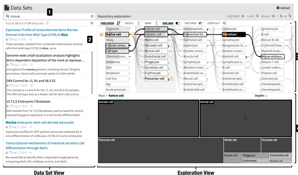
Figure 1: SATORI illustrating a query for native cells excluding precursor cells combined with a synonym keyword search for mouse. The data set view includes the search interface (1) and the list of retrieved data sets (2). The exploration view is composed of the precision-recall plot (3) and the ratio plot (4), which show the abundance and other properties of annotation terms among the retrieved data sets. The black highlighting indicates the selection of fibroblast, its parent and child terms and the associated data sets.
