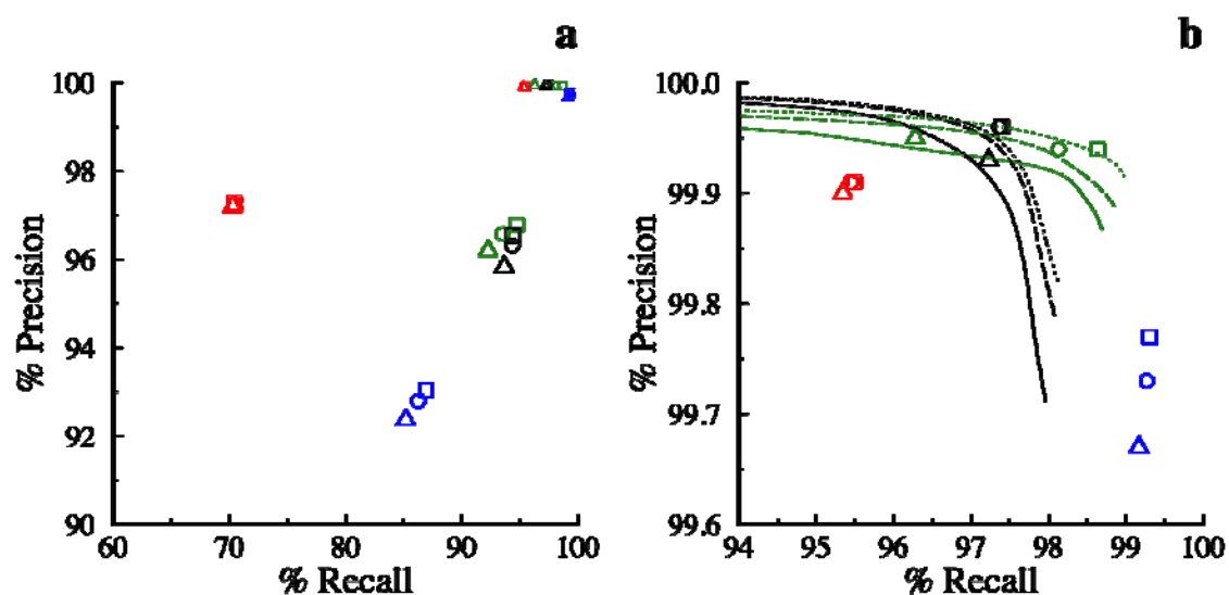
Figure 4. Precision versus recall in NA12878 evaluated against the Platinum catalogue dataset. Triangles, circles and squares respectively represent the results from 30x, 40x and 50x sequencing depth for Platypus (red), FreeBayes (blue), GATK3 (green) and Strelka (black). (a) Indels (large symbols) and SNV (small symbols) results plotted on the same axis. (b) Expansion of SNV results, also showing ROC curves for GATK3 and Strelka that reflect the trade-off of recall versus precision that is obtained by altering specific variable parameters when using the algorithms.
