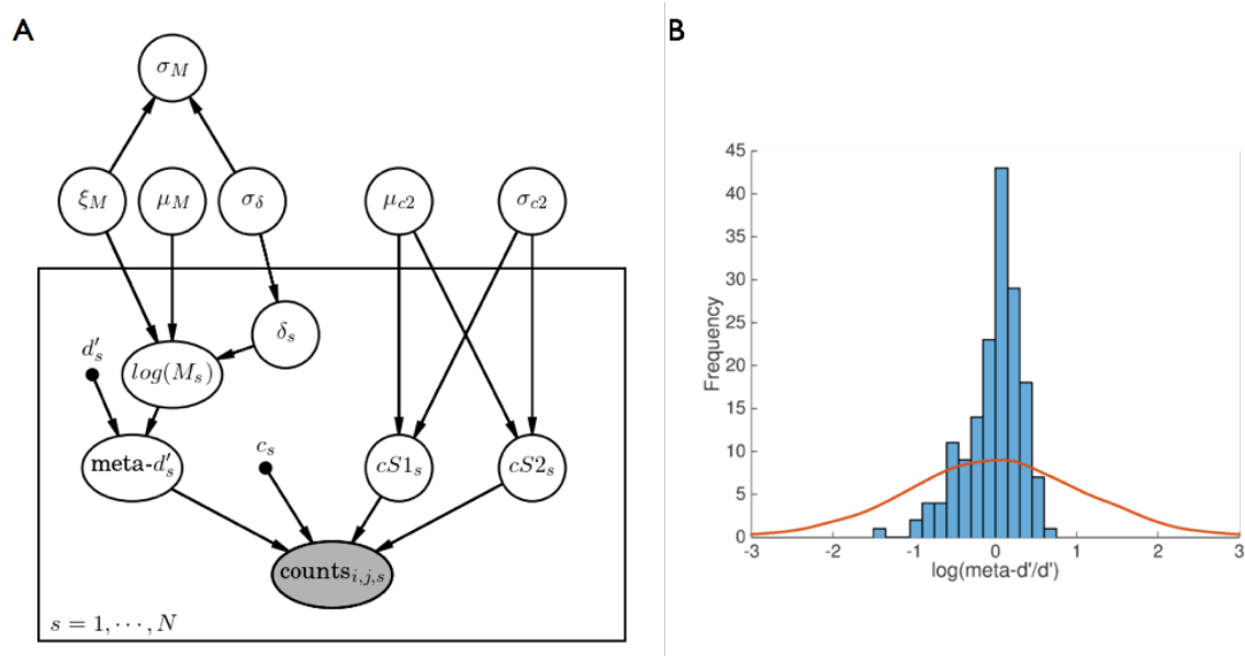
Figure 2. The hierarchical meta- d' model. A) Probabilistic graphical model for estimating metacognitive efficiency using hierarchical Bayes (HMeta- d' ). The nodes represent all the relevant variables for parameter estimation, and the graph structure is used to indicate dependencies between the variables as indicated by directed arrows. As is convention, unobserved variables are represented without shading and observed variables (in this case, confidence rating counts) are represented with shading. Discrete
