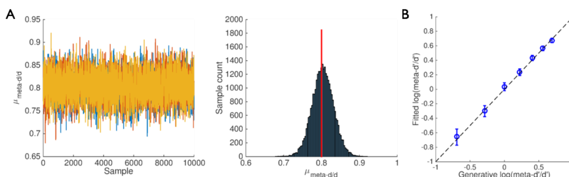
Figure 3. HMeta-d output. A) Example output from HMeta-d fit to simulated data with ground truth meta-d'/d' fixed at 0.8 for 20 subjects. The left panel shows the three MCMC chains for parameter \mu_{meta-d'/d'} ; the right panel shows the same samples aggregated in a histogram. B) Parameter recovery exercise using HMeta-d to fit data
