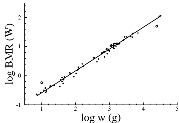
Figure 6: Marsupial mammals. The allometric relationship between the basal metabolic rate (BMR) and body mass ( w ) in marsupial mammals; with an estimated exponent of 0.75 \pm 0.01 . Data from McNab (2008), with the honey possum (left open circle) and the southern hairy-nosed wombat (right open circle) removed as outliers from the regression.
