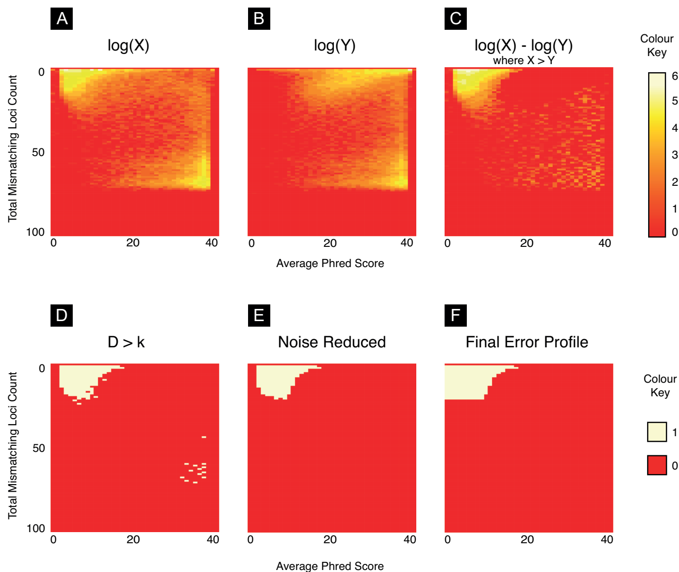
Figure 8. A: A heatmap of the joint distribution of Phred scores a mismatching loci and the number of mismatching loci ( X ). The intensities in the top left corner of the heatmap indicate an association between fewer mismatches and lower phred scores. We observe that the maximum mismatching loci is commonly \sim 75\% of the read length. This effect is caused by non-telomere reads match a the telomere sequence simply by chance B: A heatmap of the joint distribution of random loci in reads and the associated phred score ( Y ). We note that the joint distribution of reads in the upper half of the matrix is different to that in X while the lower portion is identical. C: The difference between X and Y . Referred to as D in the text. D: A binary heatmap showing all cells in D that are greater than the threshold k . We note the preponderance of cells in the upper left hand corner of the figure E: We remove noise from the figure using the methods detailed in (Supplementary Algorithm 1) F: We apply a final rule to ensure cells associated with low Phred scores are captured in the error profile (Supplementary Algorithm 2)
