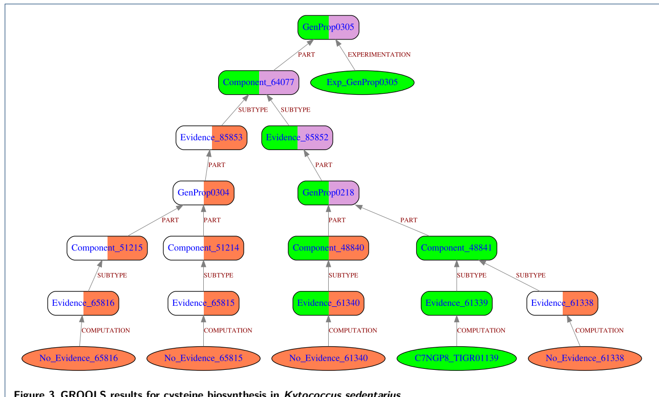
Figure 3 GROOLS results for cysteine biosynthesis in Kytococcus sedentarius .
