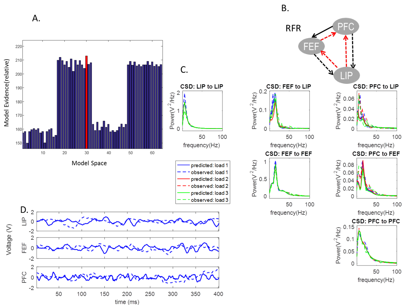
Figure 5. Contralateral WM Load Effects on FF and FB coupling in the PFC-FEF-LIP network during early delay. Plots
