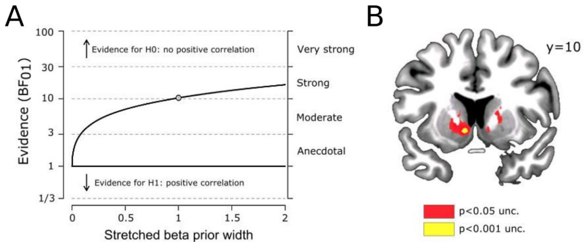
Figure 2. Control and exploratory analyses. (A) Robustness check for the Bayesian correlation analysis. This graph shows that the Bayes factor quantifying the relative evidence for the absence vs presence of a positive correlation exceeds the critical threshold of 3 for a large range of beta prior widths, even extending to strong prior beliefs in the existence of a positive correlation (values < 1 correspond to a prior biased in favor of a positive correlation, values > 1 correspond to a prior biased in favor of an absence of a positive correlation, and value = 1 corresponds to an uninformative (flat) prior as used in our main analysis). (B) A voxel-wise analysis restricted to an anatomical mask of the striatum shows that the negative correlation between sEBR and Ki values peaks in the left nucleus accumbens ([x y z] = [-8 10 -6]; p_{FWE \text{ striatal mask}} < 0.05 ).
