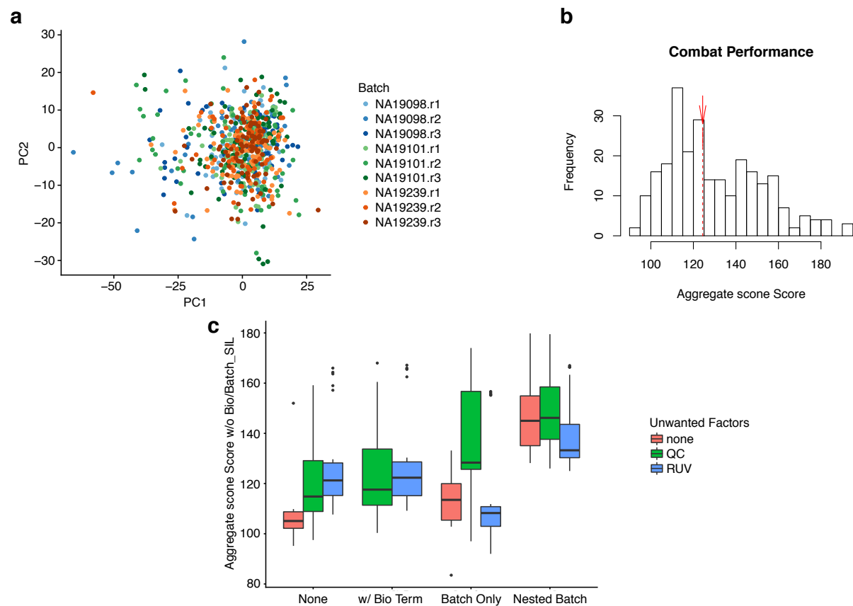
Supplementary Figure 6: Batch adjustment for the iPSC dataset [31]. (a) PCA of ComBat-normalized data. Donor-specific effects are removed. (b) Histogram of scone aggregate scores recomputed to include ComBat (red arrow). (c) Boxplot of scone aggregate scores for various normalization strategies, excluding BIO_SIL and BATCH_SIL from the aggregate score calculation.
