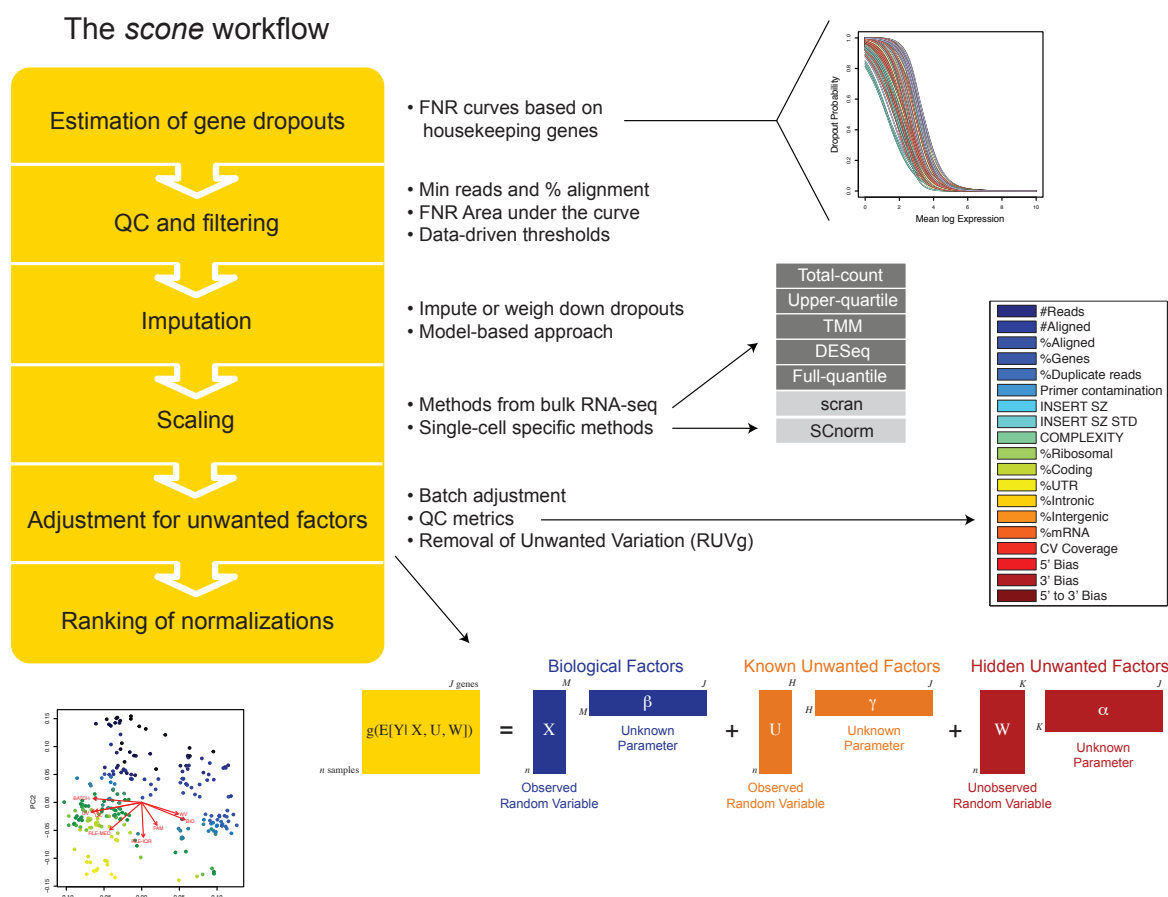
Figure 2: Schematic view of the scone workflow. The yellow box summarizes the six steps of the scone workflow. False negative rate (FNR) curves based on housekeeping genes are computed for each sample and used to infer dropouts. Using the FNR curves and the QC measures of Tables 1 or 2, low-quality samples and lowly-expressed genes are filtered out. Following an optional imputation step, the data are normalized via a combination of scaling normalization and regression-based normalization (using a linear model that includes both known and unknown covariates). Finally, the different normalization strategies are ranked according to eight performance metrics (see Methods).
