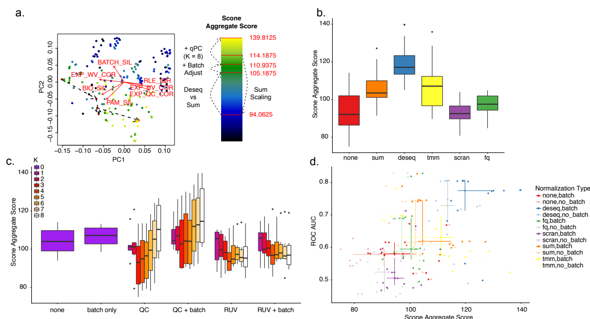
Supplementary Figure 5: scone results on the PBMC dataset [30]. (a) Biplot [33] of the scone performance metrics. Each point corresponds to a normalization workflow in the space of the first two principal components of the eight performance metrics, color-coded by the scone aggregate score (mean of eight scone score ranks). The red arrows correspond to the PCA loadings for each of the eight metrics (RLE_MED has zero length). The direction and length of an arrow can be interpreted as a measure of how much of that metric contributed to the two PCs. The points further along the direction of the arrow typically have a higher value for the corresponding metric. For instance, points in the upper-left of the biplot have a higher value for BATCH_SIL. The red circles mark the following normalization procedures (from left to right): No normalization, total-count (TC), DESeq scaling, DESeq + batch adjustment, DESeq + batch adjustment + 8 factors of QC. (b) Boxplot of scone aggregate score, stratified by scaling normalization method. (c) Boxplot of scone aggregate score, stratified by regression-based normalization method (batch, QC, and RUV). (d) ROC area under the curve (AUC) vs. scone aggregate score. Each point corresponds to a normalization workflow, color-coded by normalization method type. Methods in the top-right corner are deemed best both by scone and by our independent validation. The horizontal and vertical lines indicate, for each method type, the IQR for each variable.
