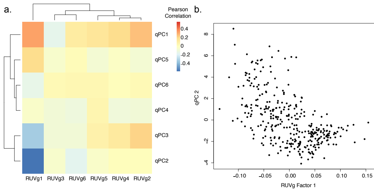
Supplementary Figure 1: Factors of unwanted variation for the Th17 dataset [25]. (a) Heatmap of matrix of Pearson correlation coefficients between RUVg factors of unwanted variation and PCs of QC measures. Rows and columns are sorted by the default ordering from the R hclust function. (b) Scatterplot of a pair of anti-correlated RUVg factor and QC PC, selected based on the correlation matrix displayed in (a).
