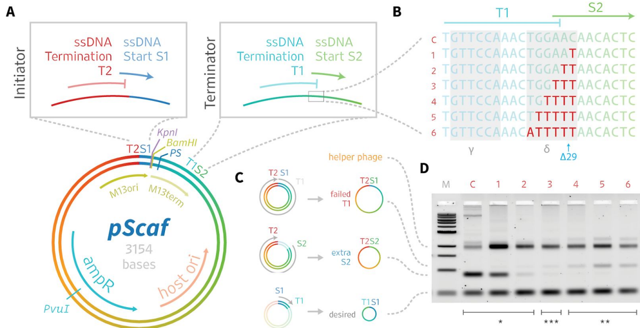
Figure 2: Construction and Optimization of the pScaf phagemid. A The pScaf phagemid is derived from the pUC18 plasmid and M13mp18 phage vectors. The phagemid includes an M13 origin of replication (M13ori) that contains ssDNA start site S1 and ssDNA termination site T2, a KpnI and BamHI cloning site, a packaging sequence (PS), and a terminator of ssDNA synthesis (M13term) containing ssDNA termination site T1 and ssDNA start site S2. The M13term sequence was adapted from the M13ori sequence by selectively deactivating the S2 ssDNA initiation function. B The ssDNA synthesis initiation and termination functions of the origin overlap. Therefore, we used a mutational screen of the \delta region to optimize the M13term performance. C Three primary species were observed: S1T2, representing failed termination at terminator T1, S2T2, representing spurious initiation at initiator S2, and S1T1, the desired product. D We analyzed the variants by agarose gel. Substituting 0–2 thymines yielded the S2T2 species (*). Substituting 4–6 bases yielded the S1T2 species (**). Substituting 3 thymines yielded the best balance between spurious S2 initiation and failed T1 termination, producing the most pure S1T1 species (***)
