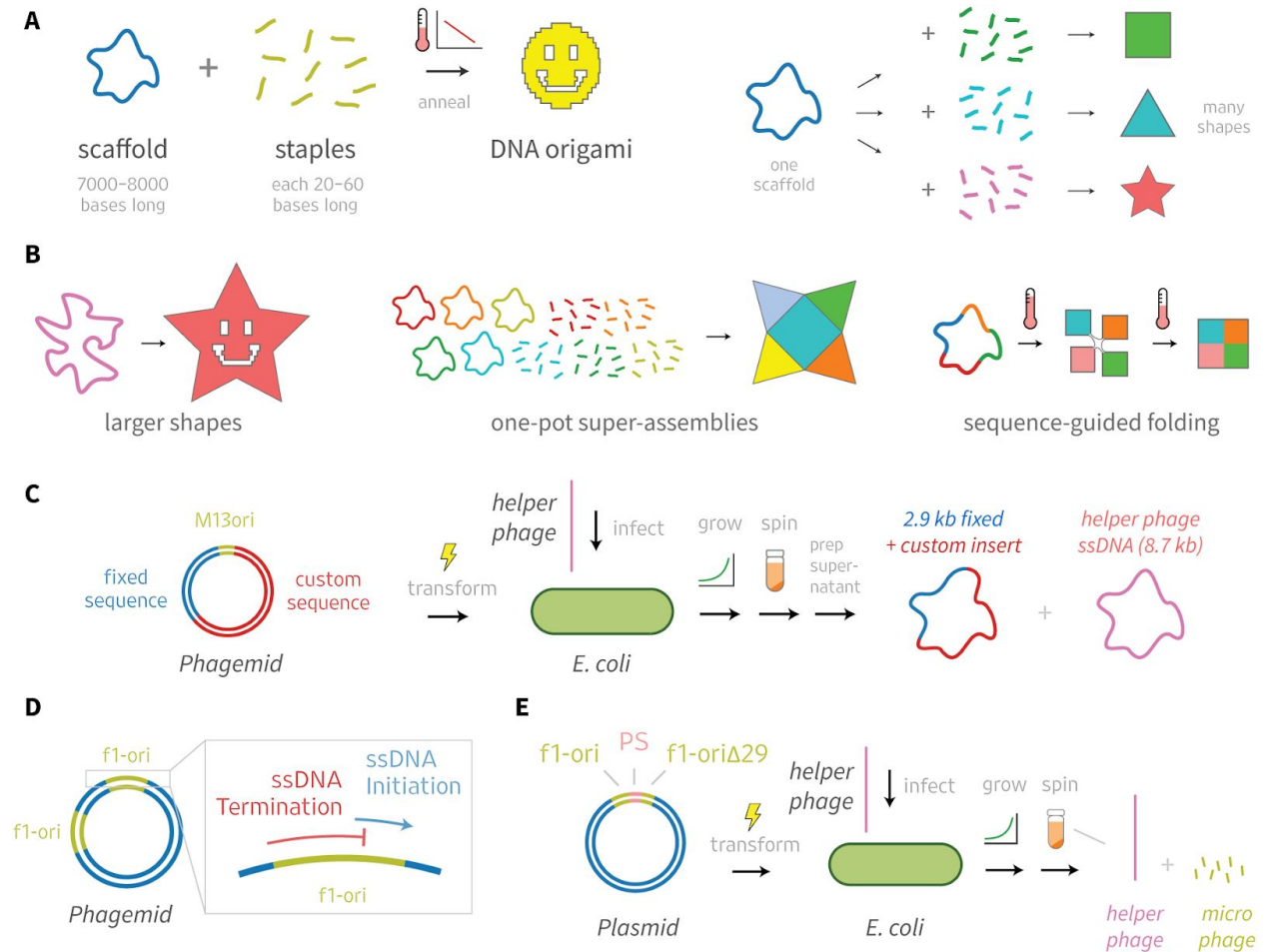
Figure 1. DNA origami design would benefit from custom scaffolds. A Many DNA origami shapes can be folded from a single scaffold. B New scaffolds will expand the space of possible designs. C Phagemids are excellent sources of scaffolds, but have multi-kilobase sequence constraints. D, E Previous studies offer hints of how these constraints could be circumvented. Dotto et al. (18) used phagemids with modified origins to show that f1-ori ssDNA initiation and termination functions overlap, but can be inactivated separately by modifying distinct sequences. Specthrie et al. (19) produced phage-like particles with ssDNA as short as 292 bases using a truncated f1-ori that acts as a terminator (f1-oriΔ29).
