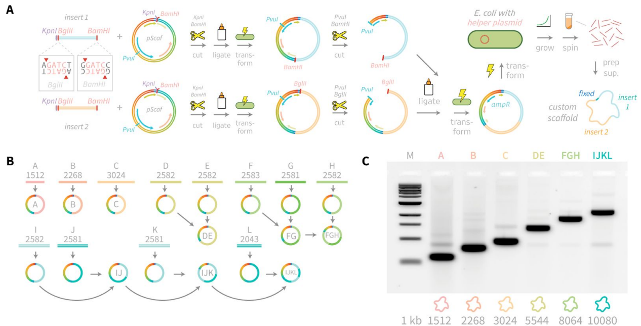
Figure 3: Cloning scheme and gel analysis of new scaffolds. A Custom sequence inserts are PCR-amplified with a forward primer containing KpnI and BglIII sites and reverse primer containing a BamHI site. Inserts up to 3 kb in length were directly transformed into E. coli bearing helper plasmid. Larger scaffolds can be assembled by iterative PvuI + BamHI digestion of the vector containing the 5' fragment, and PvuI + BglIII digestion of the vector containing the 3' fragment, followed by ligation, transformation, and miniprep. B Twelve inserts (A-L) were cloned into pScaf vector at the KpnI - BamHI site. Inserts A, B, and C were used to produce scaffolds with lengths of 1512, 2268, and 3024 bases. Larger scaffolds were assembled in multiple rounds as shown. C All scaffolds were grown in XL1-Blue cells containing helper plasmid M13cp, recovered and analyzed by agarose gel electrophoresis to determine purities ranging from 46% to 83%.
