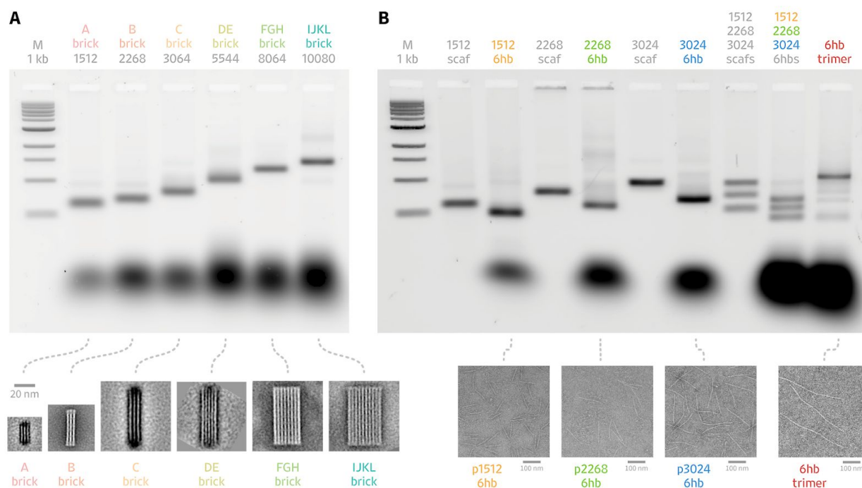
Figure 4: Folding Custom Scaffolds into DNA Origami Shapes and Assemblies. Six scaffolds of varying sizes were folded into DNA origami shapes and assemblies. Folding reactions were analyzed by gel electrophoresis, and origami analyzed negative stain transmission electron microscopy. A Brick-like DNA origami shapes were folded from scaffolds of lengths 1512, 2268, 3024, 5544, 8064, and 10080 bases. Each brick was PEG-purified and imaged by negative stain TEM. Class averages for each brick are shown, along with a 20-nm scale bar. B Scaffolds of lengths 1512, 2268, and 3024 were folded separately into six-helix-bundle (6hb) nanotubes. All three scaffolds and 6hb-staple sets were combined into one-pot reaction mixtures. When connector staples are included, the three scaffolds assemble into a 6hb trimer. TEM micrographs of the individual 6hb nanotubes and combined trimer are shown with 100-nm scale bars.
