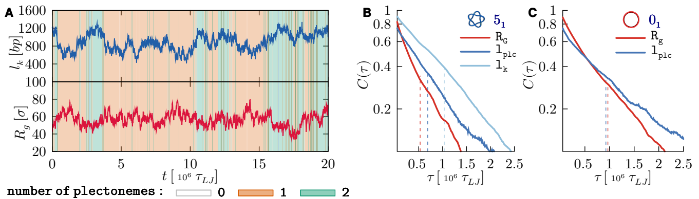
FIG. 4. (A) Typical temporal traces of the length of the knotted region, l_k and the gyration radius, R_g , from a trajectory of supercoiled 5_1 -knotted ring. The background is coloured according to the instantaneous number of plectonemes, see legend. (B) Semi-log plot of the autocorrelation functions, based on data from all trajectories, of R_g , l_{plc} and l_k of supercoiled 5_1 -knotted rings (B) and of R_g , l_{plc} for unknotted ones (C).
