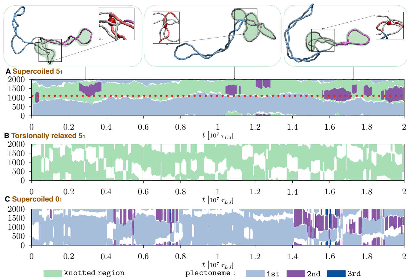
FIG. 5. Kymographs showing the typical time evolution along the ring contour of knotted and plectonemically-wound regions, see legend for colour code. The three kymographs are for: (A) supercoiled 5 1 -knotted rings, (B) torsionally-relaxed 5 1 -knotted rings and (C) supercoiled unknotted rings. The boundaries of the knotted and the main plectonemically-wound regions of case (A) are noticeable stabler than for case (B) and (C) due to persistent interlocking of multiple strands. This is illustrated in the snapshots above panel (A), where the same region at the knot-superhelix boundary (bp1000-bp1200, highlighted in red in the insets) remains entangled with other ring portions throughout the trajectory. The midpoint of this region is marked with a red bead in the insets and with a dotted red line in panel A.
