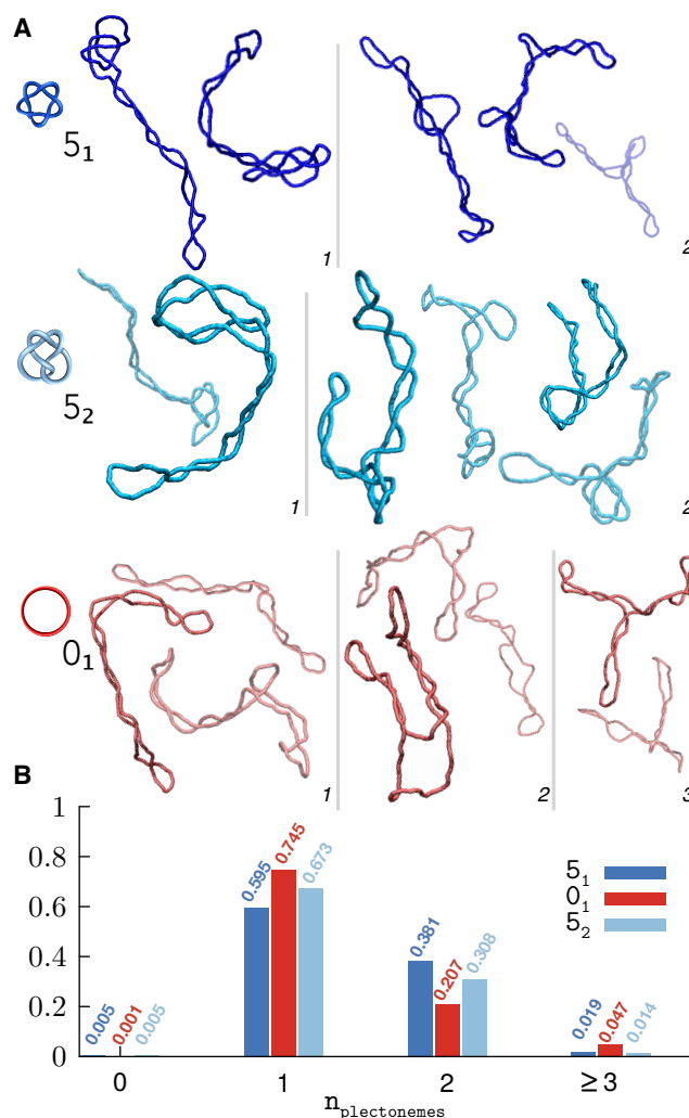
FIG. 2. a) Typical snapshots of supercoiled DNA rings for the three considered topologies. The conformers are grouped by the number of plectonemes (in italics), which increases from left to right, and are shown in colours of different saturation for visual clarity. b) Normalised histogram of the number of plectonemes observed for each topology.
