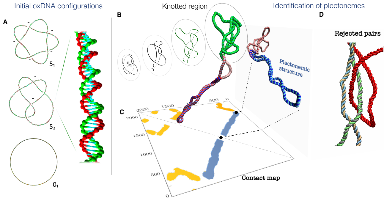
FIG. 1. (a) Initial configurations of the supercoiled double-stranded DNA rings for the three considered topologies, 0_1 , 5_1 and 5_2 . The latter two are left-handed, i.e. the topological sign of their projected crossings is negative, as indicated. The 5_1 and 5_2 snapshots have been edited to highlight the over- and underpasses, see Supplementary Fig. S1 for the unedited versions. The mesoscopic structural representation of the oxDNA model is illustrated in the inset, which shows a magnified portion of one of the rings. The twist was uniformly adjusted for each of the three cases to yield the same level of negative supercoiling (-5%). (b-d) Identification of the knotted and the plectonemically-wound regions for a typical 5_1 -knotted supercoiled conformation, shown in the foreground. (b) The knotted region (green) is the shortest portion that, after suitable bridging of the termini, has the same ( 5_1 ) topology of the entire ring. (c) The plectonemically-wound region (blue) is found by using the contact map to identify long superhelical regions ending in a short apical loop and that are free of cis or trans entanglement, as in the case of panel (d).
