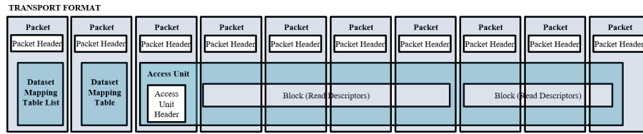
Figure 4: Key components of the MPEG-G Transport Format.
