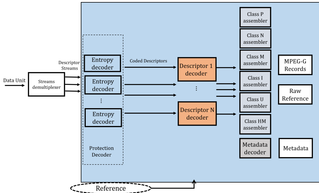
Figure 7: Simplified MPEG-G decoding process from a Data Unit to the normative output.
