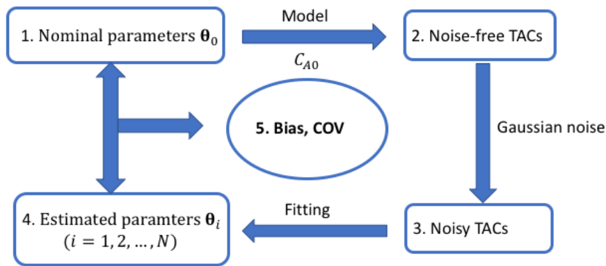
Figure 3. Flowchart of the practical identifiability analysis using Monte Carlo simulation.
