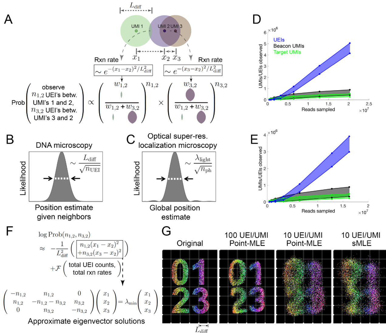
Fig. 3. Image inference from DNA microscopy data. (A) Modeling diffusion of amplifying UMIs as isotropic across length scale L_{diff} allows the likelihood of a UMI-position solution to be evaluated given observed UEI counts. (B,C) Uncertainty in DNA vs. super-resolution microscopy. Given its reacting partners' positions, DNA microscopy (left) defines a UMI's uncertainty as a physical length-scale (DNA diffusion distance, L_{diff} ) divided by the square-root of the number of individual quanta measured (UEIs) in a manner analogous to quanta (photons) in super-resolution microscopy (right). (D,E) Rarefaction of UMI and UEI data. Shown are curves with an upper-bound, indicating total UMI/UEI counts, and a lower-bound, indicating those from the final pruned UEI matrix, for samples 1 (D) and 2 (E). (F) The sMLE algorithm uses eigenvector solutions to part of the position-probability function to identify a linear basis for the solution to the full likelihood function. (G) sMLE enhances performance in free-diffusion simulation tests. From left: original image, results from point-MLE on simulated images with 100 or 10 UEIs/UMI, and from sMLE with 10 UEIs/UMI.
