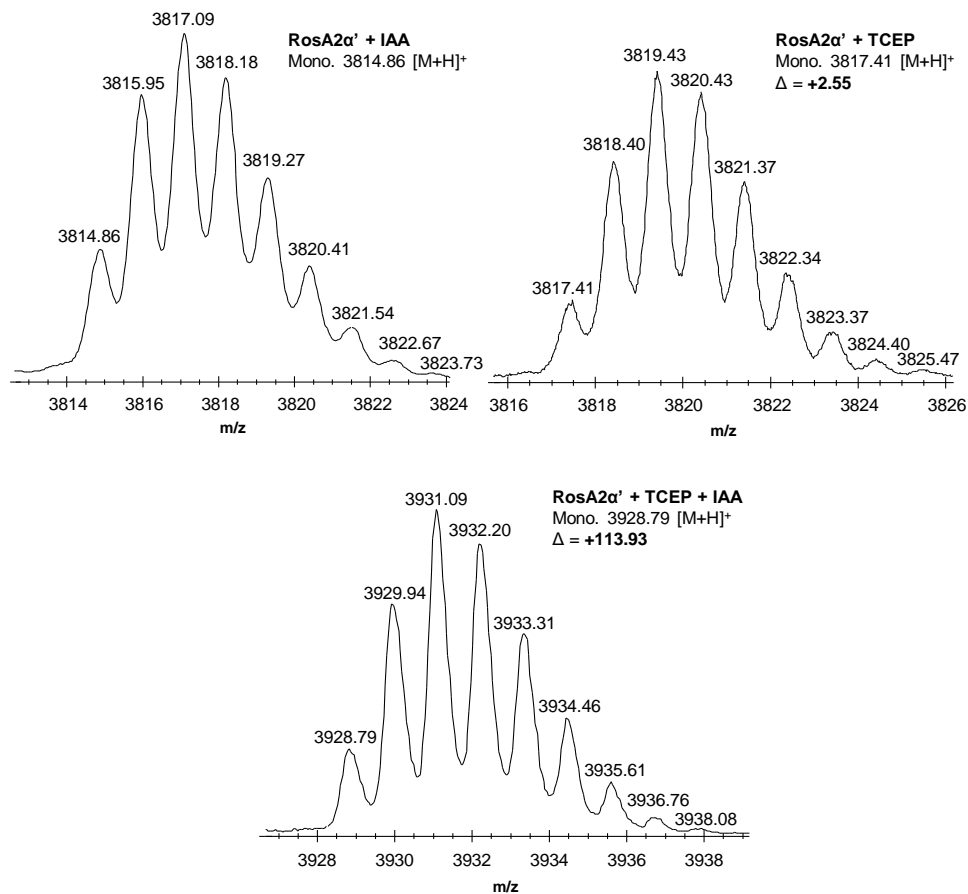
Figure S2. Related to Figure 3. Alkylation assay of RosA2α' and analysis with high-resolution MALDI TOF MS. His 6 -mRosA2 was subjected to GluC digestion and given treatment with IAA only, TCEP only, and TCEP followed by IAA. (A) RosA2α' treated with IAA alone did not lead to any change in mass. (B) RosA2α' when treated with TCEP led to an increase of mass by ~2 Da. (C) Two carbamidomethylations (~ +114 Da) were observed upon reduction with TCEP followed by IAA treatment.
