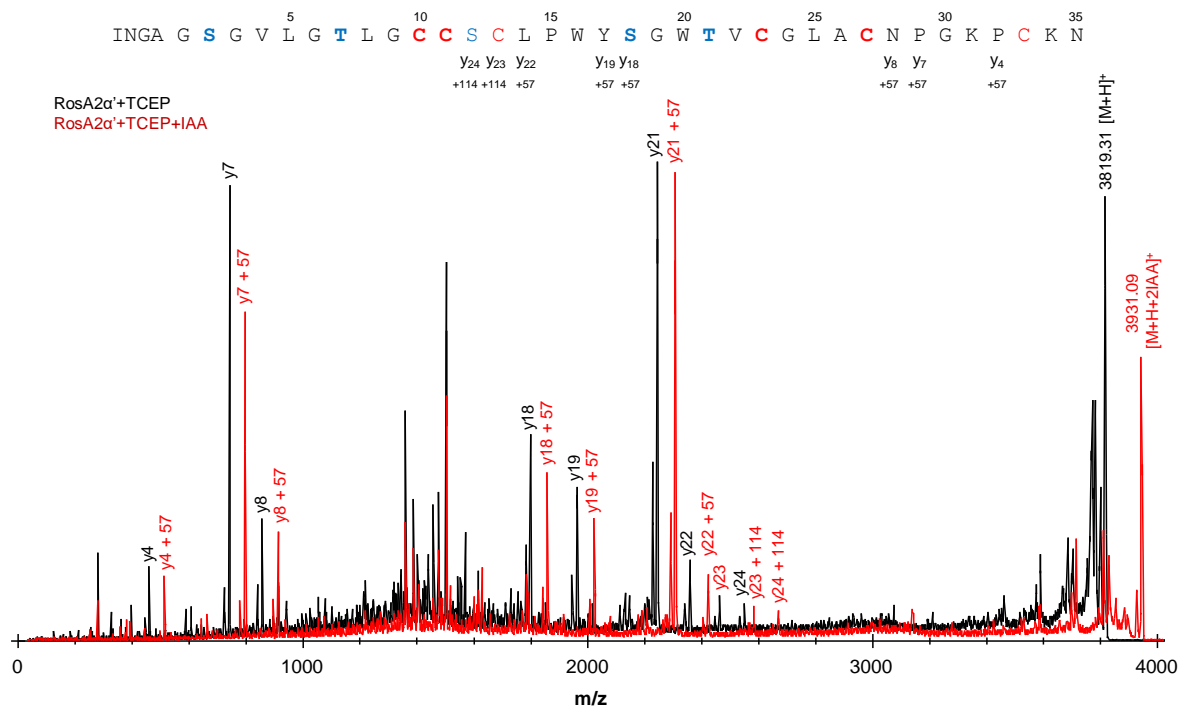
Figure S4. Related to Figure 3. Tandem MS analysis of alkylated and non-alkylated RosA2 \alpha' . Selective y ions are labelled for indicating the position of alkylation. Fragment ion y_4 to y_{22} indicate one carbamidomethylation at Cys33 and y_{23} indicate another at Cys13. Residues in bold are modified by RosM.
