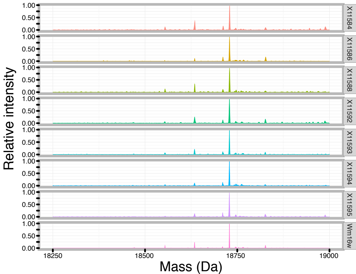
Supplementary Figure 2: Individual intact mass spectra from Wistar Han and Brown Norway animals.
