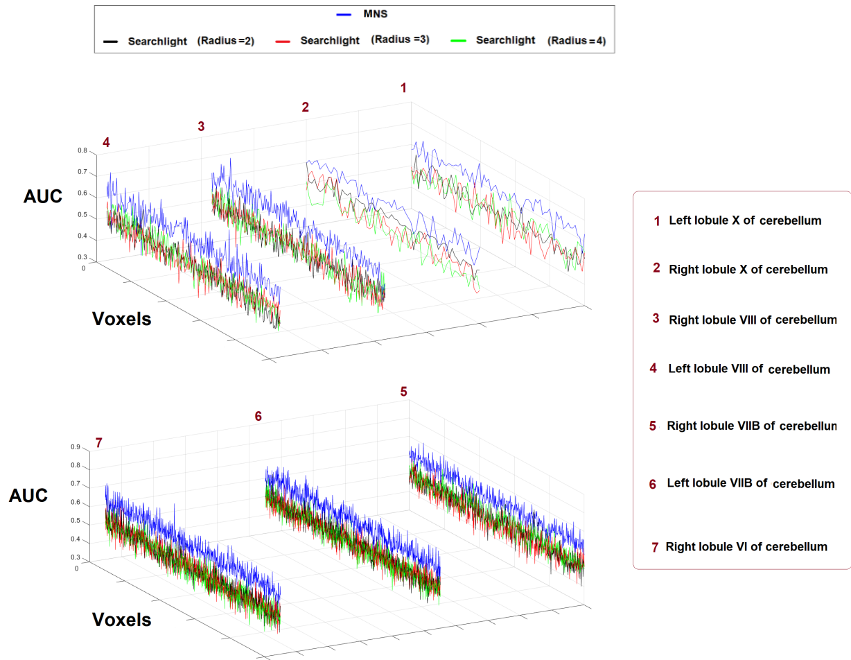
Figure 1: Test AUC for classification with decision tree of the MNS algorithm and the searchlight method with different search radii for different cerebellar regions per AAL using the ABIDE dataset.
