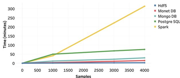
Figure 5a: Times for extracting a cross-section of a number of contiguous samples and 1 million contiguous markers
