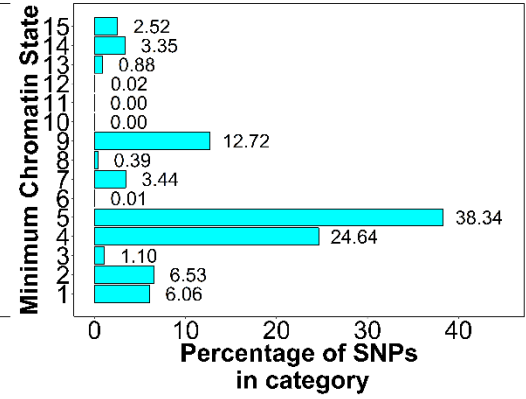
Minimum Chromatin State of SNPs found in independent genomic risk loci
