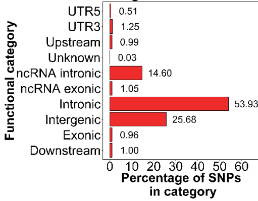
Functional category of SNPs in independent genomic risk loci
