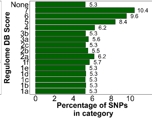
RDB Score of SNPs found in independent genomic risk loci
