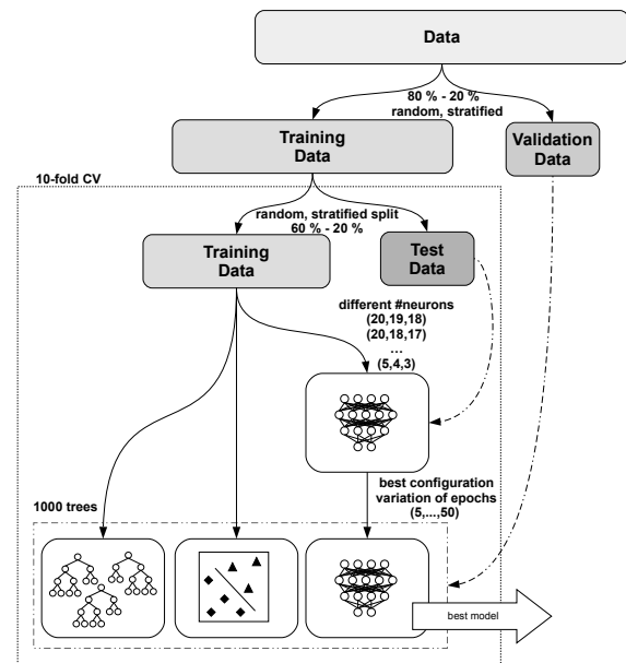
Figure 4: Development of prediction models.
