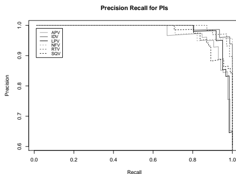
Figure 8: Precision-recall curves.
