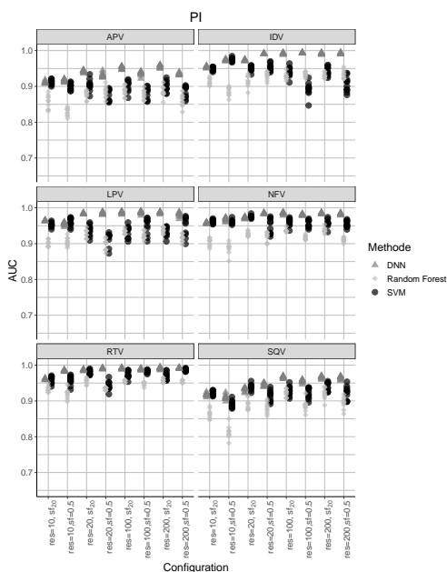
Figure 6: AUCs for PIs. Results from with different training splits and different configurations valuated with the validation data. Triangle: DNN; raute: RF; circle: SVM.
