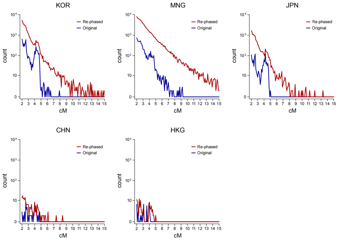
Supplementary Figure 3. Length distribution of shared IBD tracts between the two individuals in each population. Distributions of shared IBD tracts which were computed using the original and the re-phased haplotypes were displayed separately. Lengths of the shared IBDs are different by populations, but consistently increased in the re-phased haplotypes across all.
