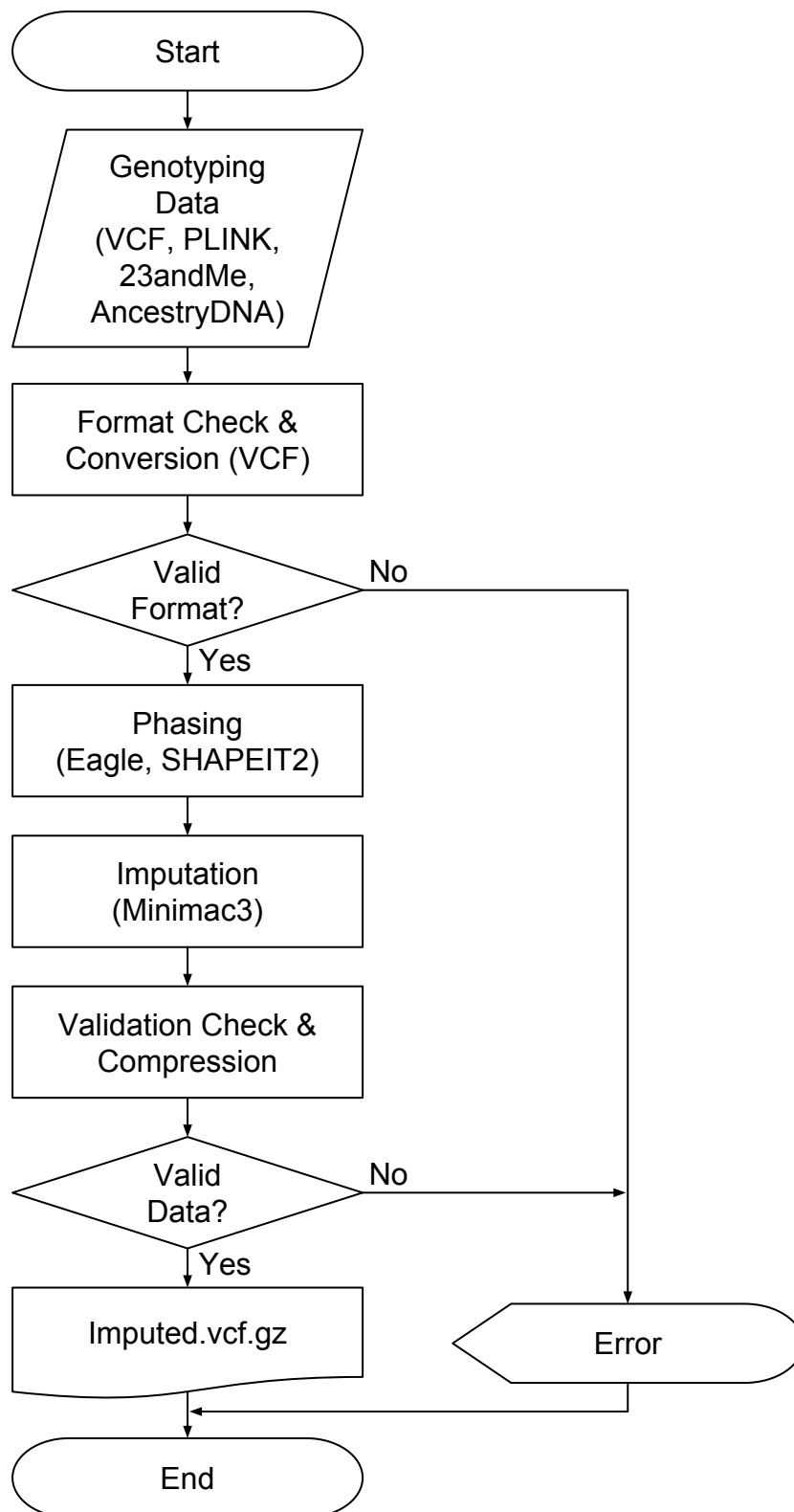
Supplementary Figure 5. The flow chart of the pipeline consisting of four major steps for NARD imputation server.
