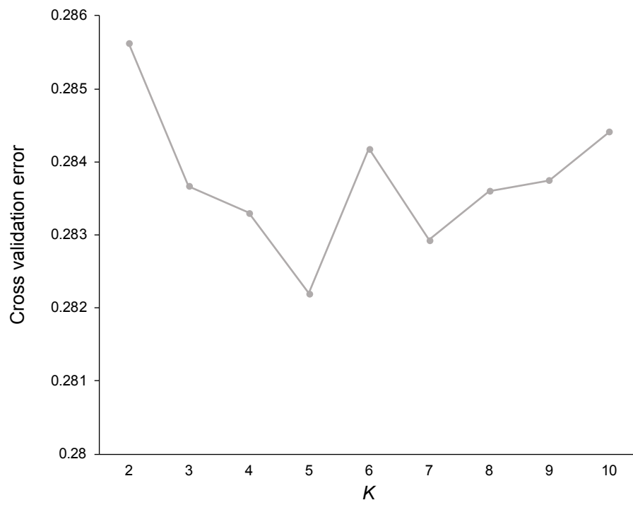
Supplementary Figure 6. The cross-validation error inferred by ADMIXTURE algorithm.
