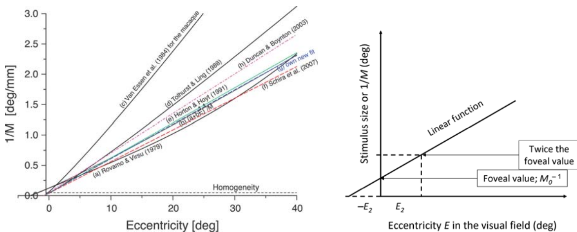
Figure 1. A. The inverse of the cortical magnification factor, or – equivalently – the size of a patch in the visual field that projects onto a patch of constant size in the cortex, as a function of eccentricity in the visual field (Fig. 9 in Strasburger et al., 2001, reproduced for illustrating the text). All functions show a mostly linear behavior. Their slope is quite similar, with the exception of Van Essen et al.’s (1984) data for the macaque; other data show similar slopes between human and monkey (e.g. Oehler, 1985). B. An illustration of the E_2 concept.
