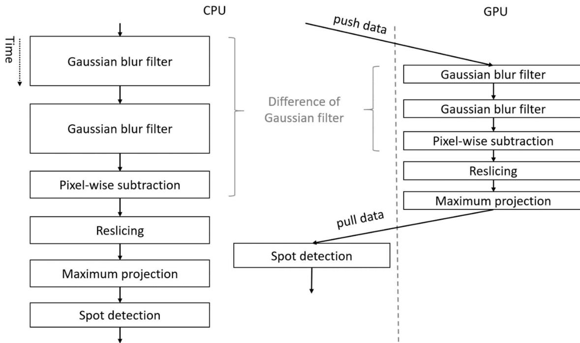
Supplemental Figure 1: Sequence diagram visualising that the GPU-accelerated workflow ends earlier even though data has to be pushed to GPU memory and pulled back. Difference-of-Gaussian filtering and a cylindrical maximum projection pre-process the image stack before spot detection is used to estimate nuclei count on the surface projection of a Drosophila embryo.
