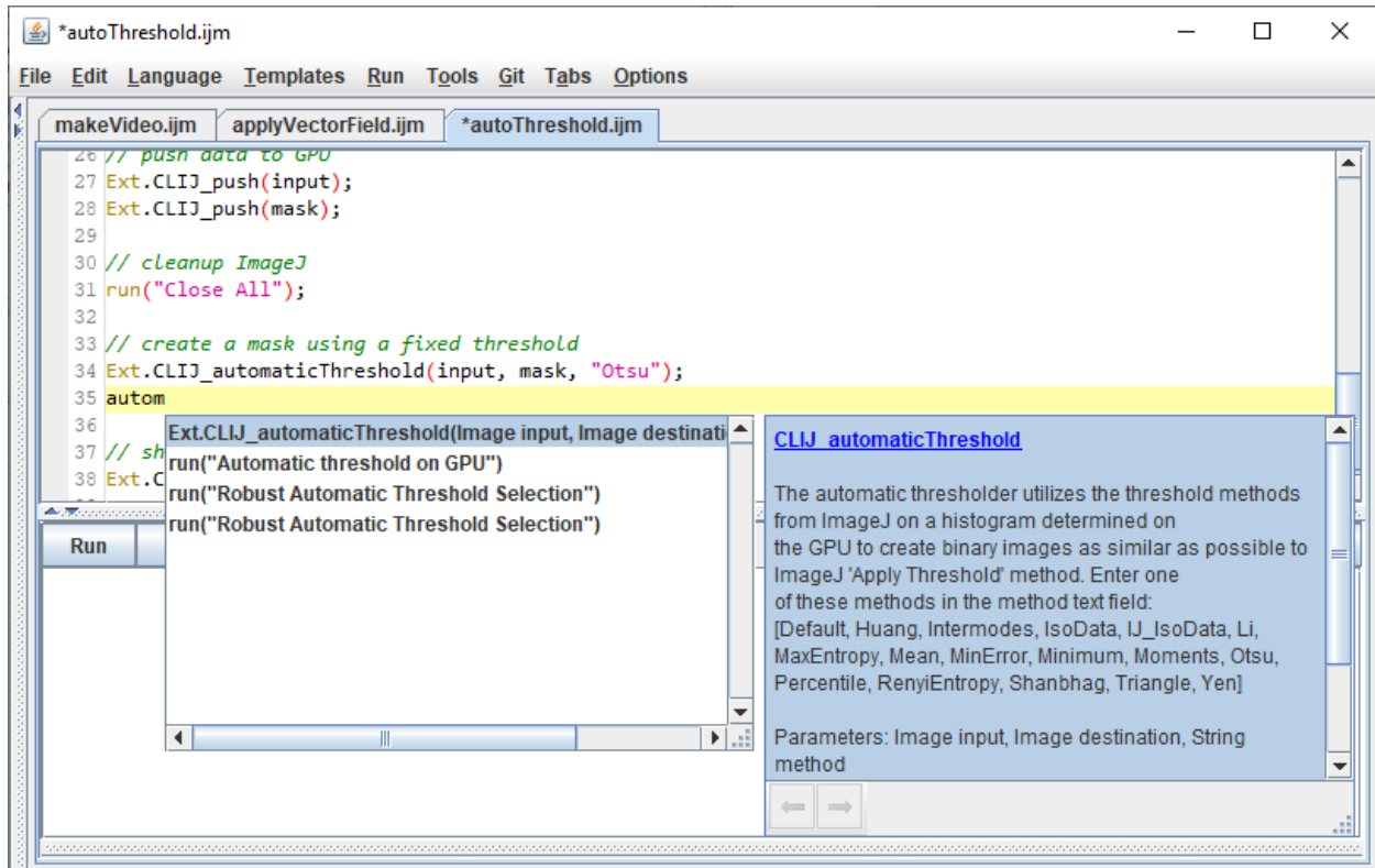
Supplementary Figure 3: Fijis script editor has been enriched with CLIJ specific auto-completion and online-help enabling users to assemble GPU-accelerated workflows without the need for reading the full documentation of CLIJ.
