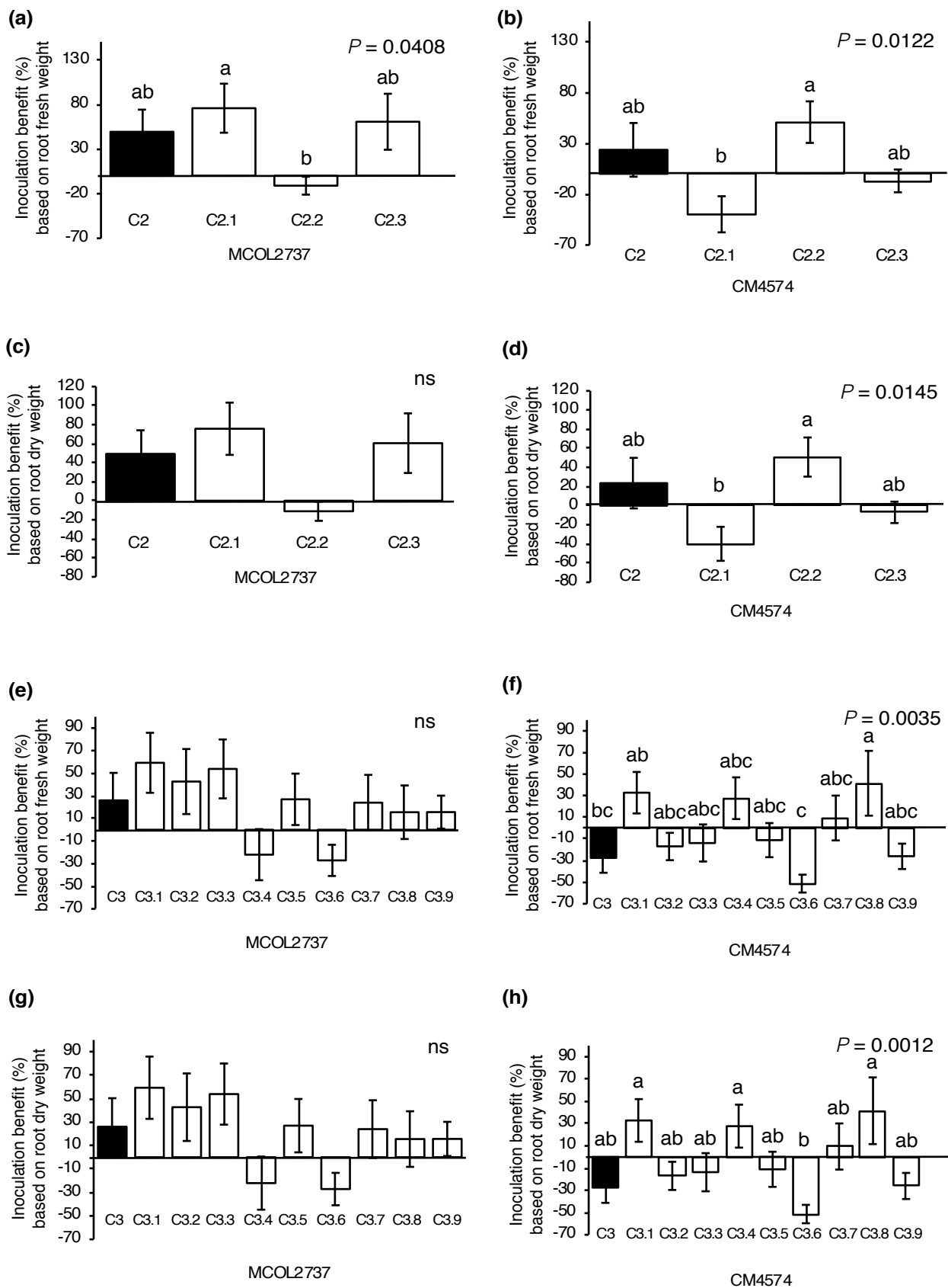
Supplementary figure 3. Inoculation benefit based on root fresh and dry weight of cassava cultivars MCOL2737 and CM4574 inoculated with the parental R. irregularis isolate C2 and its clonal progeny and the parental R. irregularis isolate C3 and its clonal progeny averaged over the two trials in experiment 4. Parental isolate treatments shown in black and progeny treatments unshaded. Bars represent +1 S.E. Different letters above bars represent significant differences ( P \leq 0.05 ) according to a Tukey honest significant difference test. See Supplementary table S4 for a summary of statistical analyses and Supplementary information for full details of all statistical tests.
