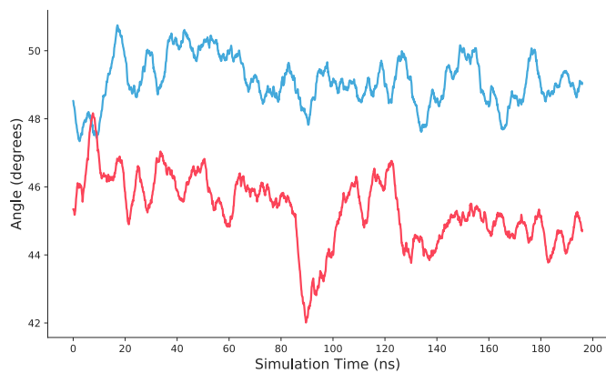
Figure S1: Molecular Dynamics of WT (red) vs R268G Mutant forms of FH (blue). Shown is the angle between residues 158, 268, 331.
