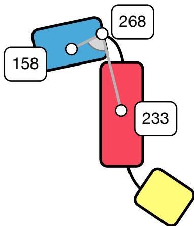
Figure S1: Molecular Dynamics of WT (red) vs R268G Mutant forms of FH (blue). Shown is the angle between residues 158, 268, 331.
