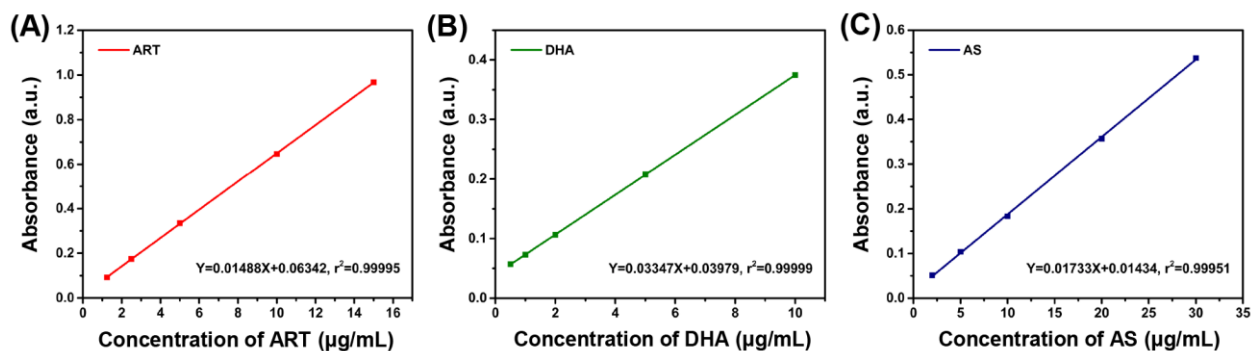
Supplementary Figure S2. Standard curves of (A) ART, (B) DHA, and (C) AS concentration.
