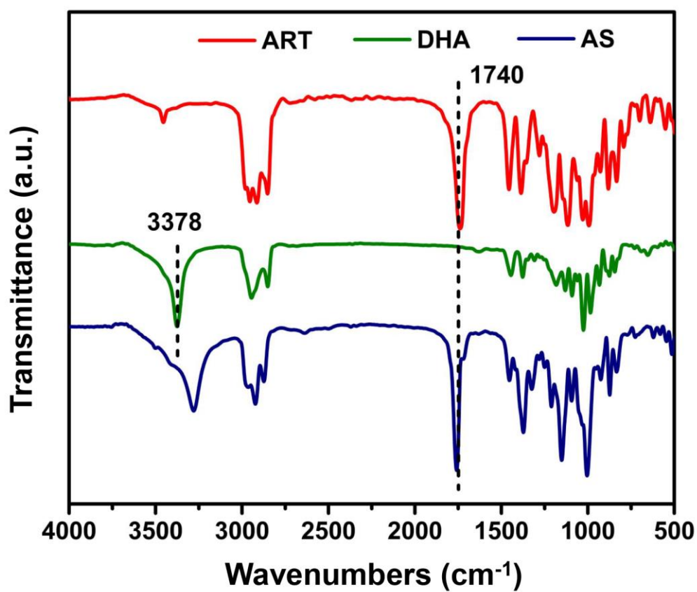
Supplementary Figure S1. FT-IR spectra of ART, DHA, and AS.
