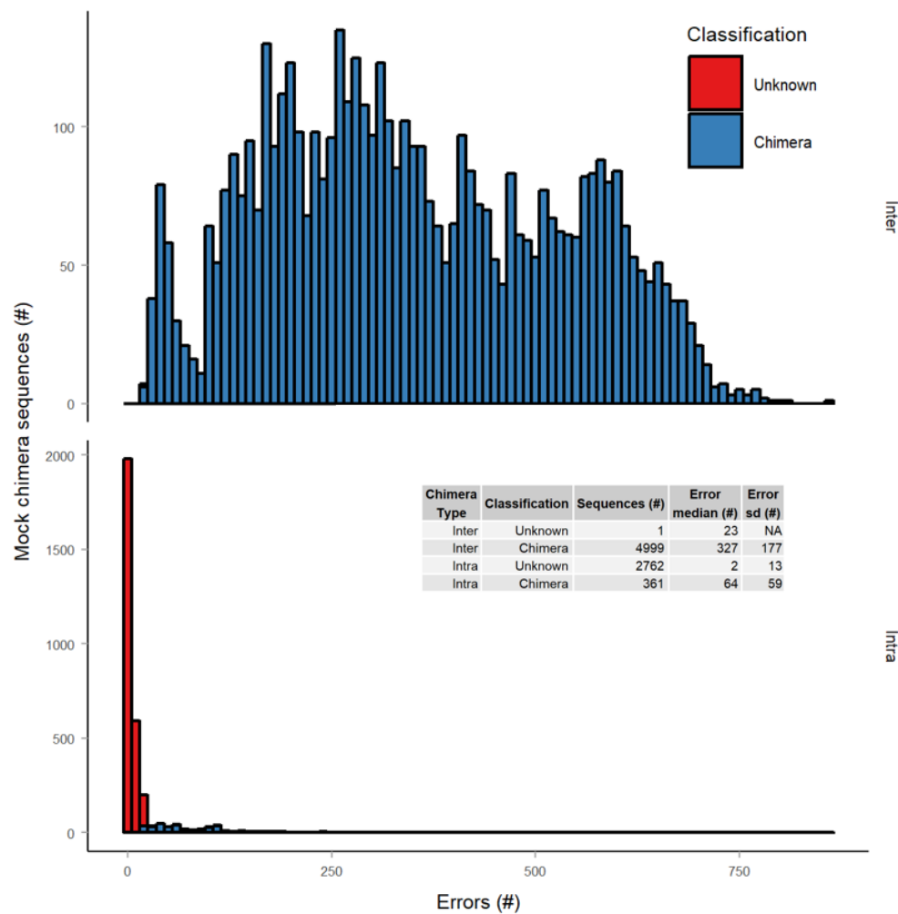
35 Figure S8: Validation of chimera detection. Chimera detection is notoriously difficult in the presence of sequencing errors and false positives/negatives are unavoidable 1 . For detecting 40 chimeras in the ZymoBIOMICS Microbial Community DNA Standard rRNA operon data we used uchime2_ref in sensitive mode. To validate that closely related chimeras could be identified with this approach, we generated a chimera dataset from the reference sequences in the mock microbial community, which had between 1 to 842 bp differences to the closest matching references. 99.98% 45 of the inter-species chimeras (n = 5000) were detected along with 11.6% of the intra-species chimeras (n = 3123). The plot shows the test results; the data is divided by inter- and intra-species chimeras, and the x-axis shows the number of differences between the chimera and closest matching reference and the y-axis shows the number of chimeras. It is mainly chimeras with few SNPs that are not classified. The chimera detection method proved to generate false positives when contaminating sequences were present. Hence, detected chimeras were validated by manual inspection (see Figure S2).
