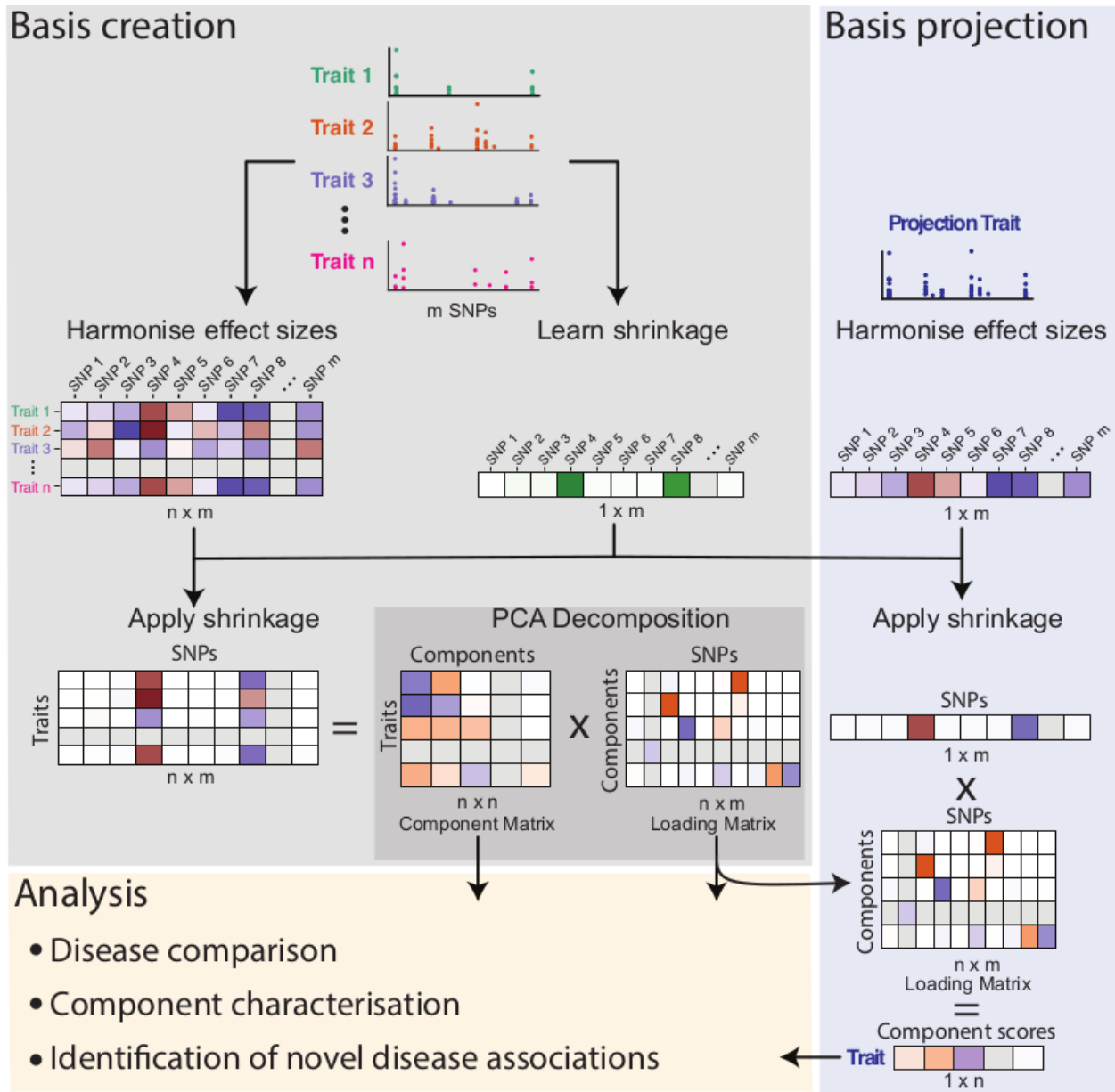
Figure 1: Schematic of basis creation and projection. Basis creation: GWAS summary statistics for related traits are combined to create a matrix, M ( n \times m ), of harmonised effect sizes ( ) and a learned vector of shrinkage values for each SNP. After multiplying each row of M by the shrinkage vector, PCA is used to decompose M into component and loading matrices. Basis projection: External trait effects are harmonised with respect to the basis, shrinkage applied and the resultant vector is multiplied by the basis loading matrix to obtain component scores which can then be used for further analyses.
