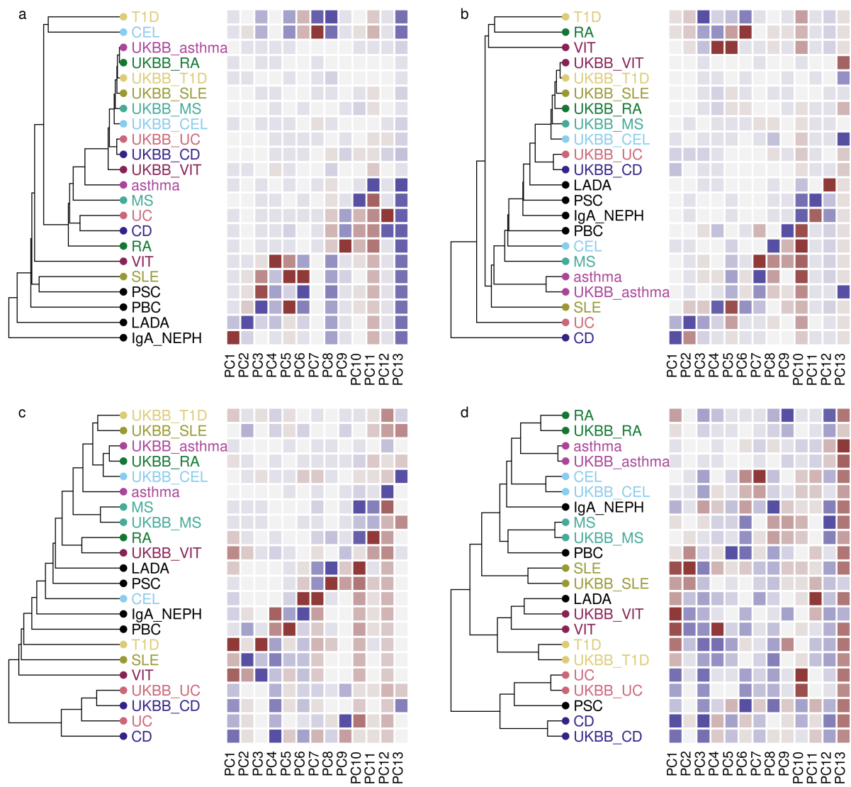
Figure 2: Hierarchical clustering of basis diseases and their UKBB counterparts in basis space a un-weighted basis constructed using b hard-thresholded, LD-thinned basis constructed using Z scores c hard-thresholded, LD-thinned basis constructed using d basis constructed using continuous shrinkage applied to . Heatmaps indicate projected for each disease on each component PC1-PC13, with grey indicating 0 (no difference from control), and darker shades of green or magenta showing departure from controls in one direction or the other. GWAS datasets: T1D = type 1 diabetes, CEL= celiac disease, asthma, MS =multiple sclerosis, UC =ulcerative colitis, CD = Crohn’s disease, RA =rheumatoid arthritis, VIT =vitiligo, SLE =systemic lupus erythematosus, PSC=primary sclerosing cholangitis, PBC=primary biliary cholangitis, LADA=latent autoimmune diabetes in adults, IgA_NEPH= IgA nephropathy. UKBB_ prefixed diseases correspond to self reported disease status in UK Biobank.
